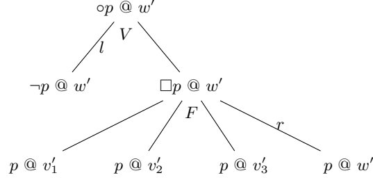
Fig. 3: Game tree for the semantic game for the formula \circ p at w' in model M' .
