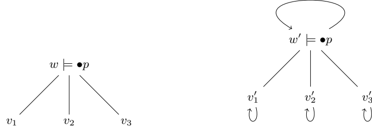
(a) The model M without the reflexive arrows. (b) The model M' with the reflexive arrows.
