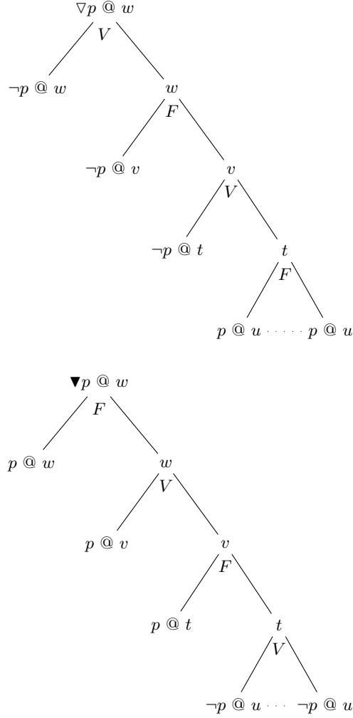
Fig. 5: The game trees for the formulas \nabla p and \blacktriangledown p at state w , respectively, where v \in R[w] , t \in R[v] , u \in R[t] .
