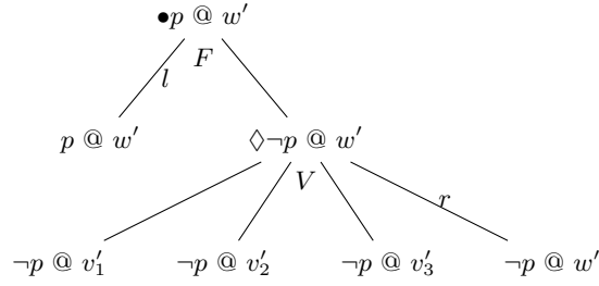
(b) The game tree based on M' .
