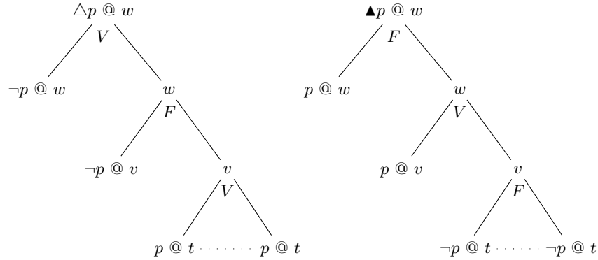
Fig. 4: The game trees for the formulas \triangle p and \blacktriangle p at state w , respectively, where v \in R[w] and t \in R[v] .
