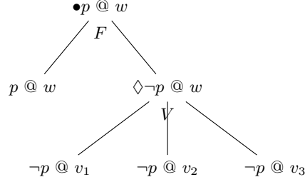
(a) The game tree based on M .
