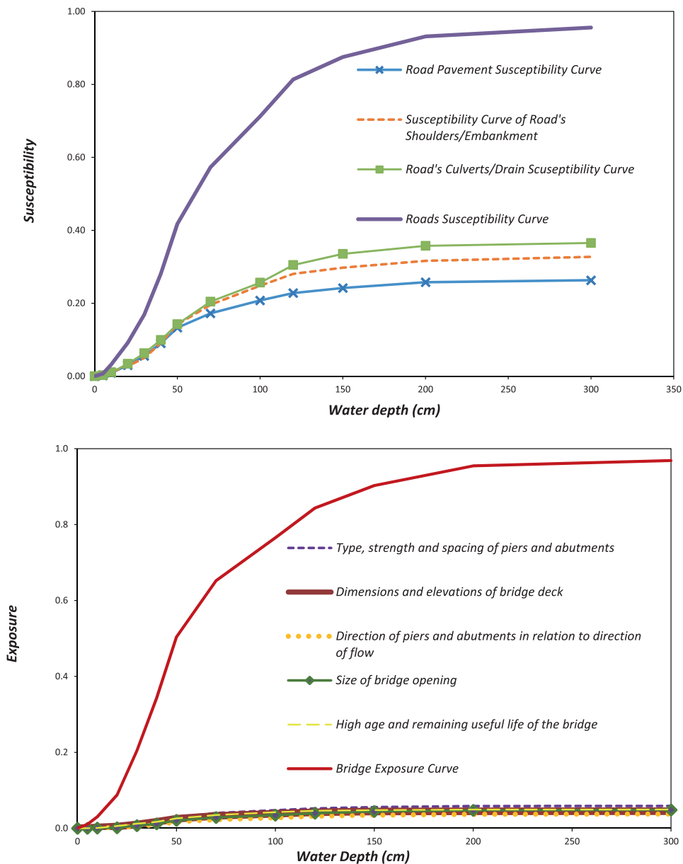
FIGURE 12 The indicator-based roads susceptibility (above) and bridge exposure (below) curves for Sarajevo, Bosnia.
