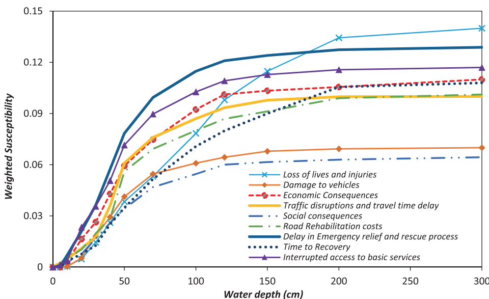
FIGURE 11 Weighted susceptibility curves for each indicator for one single component of the road infrastructure in Sarajevo, Bosnia.
