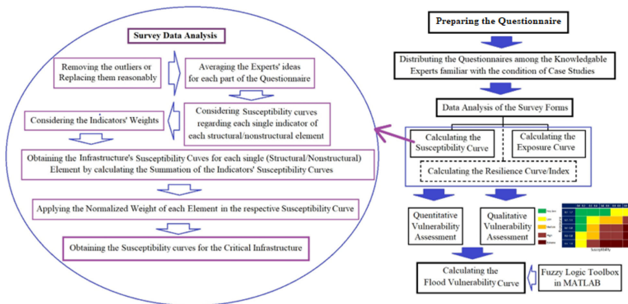
FIGURE 4 Flowchart shows the analysis of the questionnaire to obtain critical infrastructures flood vulnerability curves.
