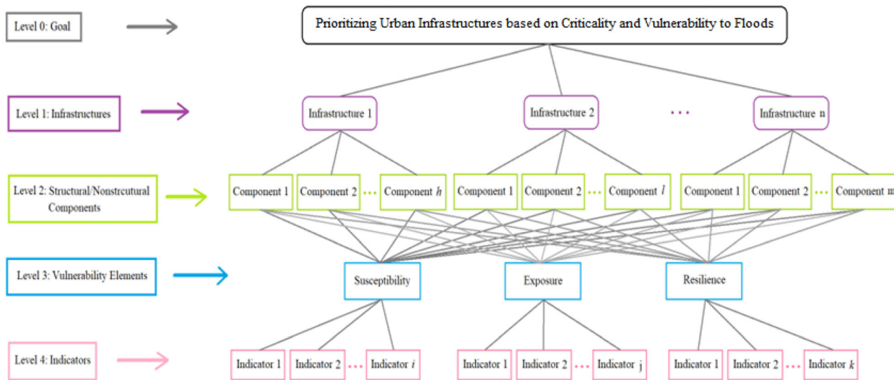
FIGURE 9 The proposed MCDM framework for calculating the criticality values (based on vulnerability to floods).
