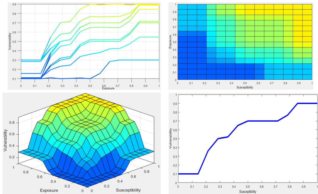
FIGURE 8 Fuzzy rules defined using Fuzzy Logic Toolbox in MATLAB.
