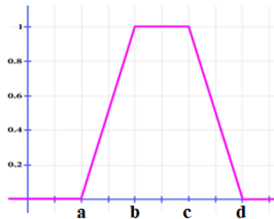
FIGURE 7 Trapezoidal membership function curve (Setiawan et al., 2020).
