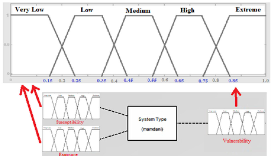
FIGURE 6 Definition of inputs, outputs, and their membership functions.
