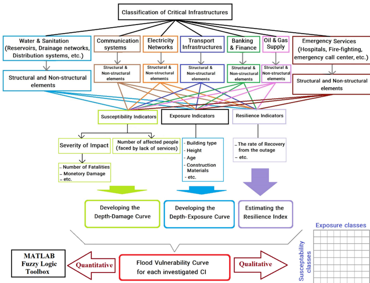
FIGURE 3 The proposed framework for classifying the Most Vulnerable Urban Infrastructures to flooding. CI, critical infrastructures.
