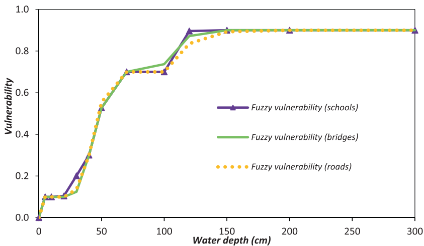
FIGURE 13 Vulnerability curves for roads, bridges (top), and schools (bottom) in Sarajevo, Bosnia.
