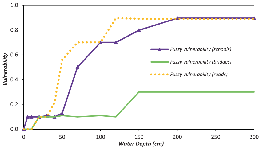
FIGURE 14 Fuzzy vulnerability curves for roads, bridges, and schools in Berat, Albania.
