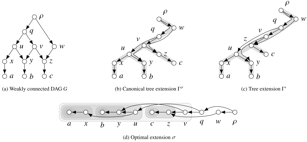
Fig. 4. (a): Weakly connected, rooted DAG G . (b): Optimal canonical tree extension \Gamma^\sigma with scanwidth 3, attained at the vertex v . (c): Non-canonical tree extension \Gamma' with scanwidth 4, attained at the vertex z . (d): Optimal extension \sigma with scanwidth 3, attained at the vertex v . For each i \leq 8 , the outermost grey shaded areas containing only vertices belonging to \sigma[1 \dots i] depict the weakly connected components of G[1 \dots i] . For i \geq 8 , G[1 \dots i] is weakly connected and therefore consists of just one component.
