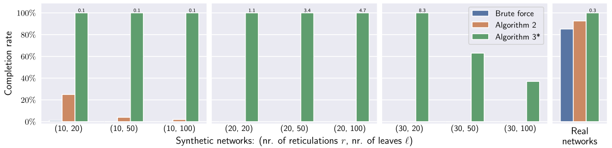
Fig. 16. Performance of the exact algorithms. For each algorithm, the completion rate, calculated as the number of instances per data set where the algorithm successfully computed the scanwidth within 60 seconds, is shown. If the rate is 100%, the average running time in seconds is also depicted. The figure contains results for each of the nine subsets of the synthetic data and one for the real dataset. The different colors indicate the different algorithms. In all cases, the decomposition algorithm was also applied. The asterisk in the legend indicates that we repeatedly applied Algorithm 3 as outlined in the proof of Corollary 4.12, since the algorithm itself only solves the fixed-parameter version of the problem.
