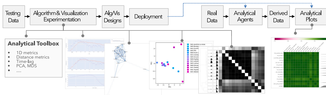
Fig. 5. The analytical support team develops and experiments with different analytical algorithms and visual representations (top left) and selects some designs to be deployed on the VIS infrastructure by the generic support team (top right). The lower part of the figure shows examples of analytical visualisations for time series analysis, including time-lag plot, force-directed graph, scatter plot, and heatmap matrix.
