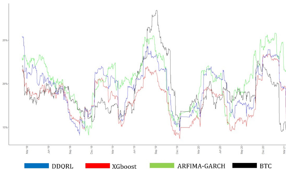
FIGURE 2 | Rolling standard deviations obtained by each strategy. [Colour figure can be viewed at wileyonlinelibrary.com ]
