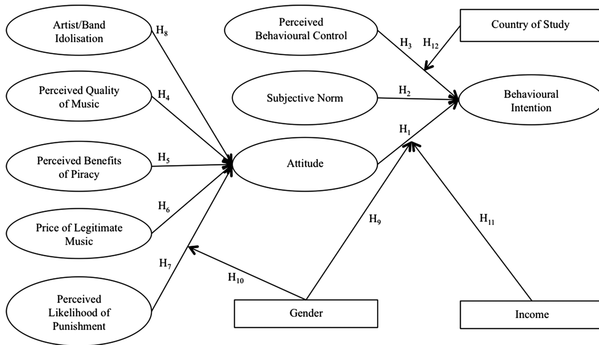
Figure 1. Conceptual model.
