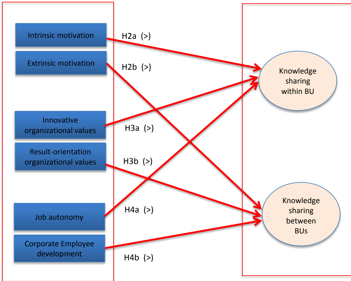
Figure 1. Theoretical model
