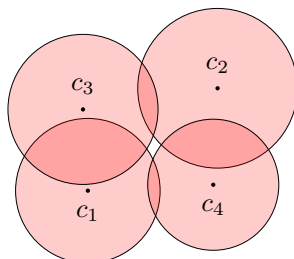
■ Figure 1 Disk realization of a K_{2,2} . As the centers are positioned, it is impossible that the two non-edges are between the disks 2 and 3, and between the disks 1 and 4 (or between the disks 1 and 3, and between the disks 2 and 4).
