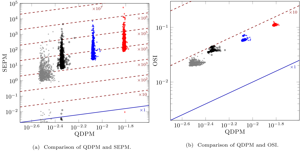
Fig. 5. Comparisons on random games with 5000 positions.
