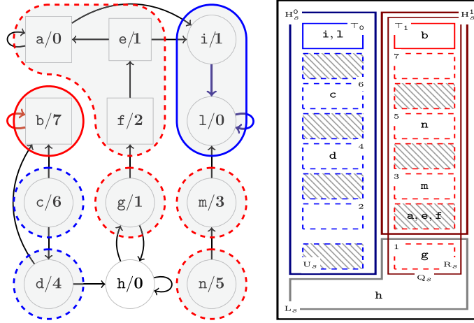
Fig. 4. A game and a corresponding state representation.
