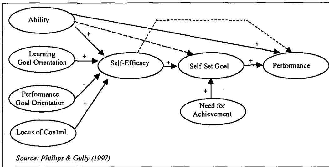
Figure 3.12 Theoretical Model
