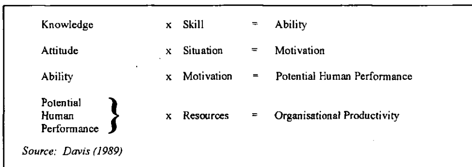
Figure 3.6 Organisational Productivity
