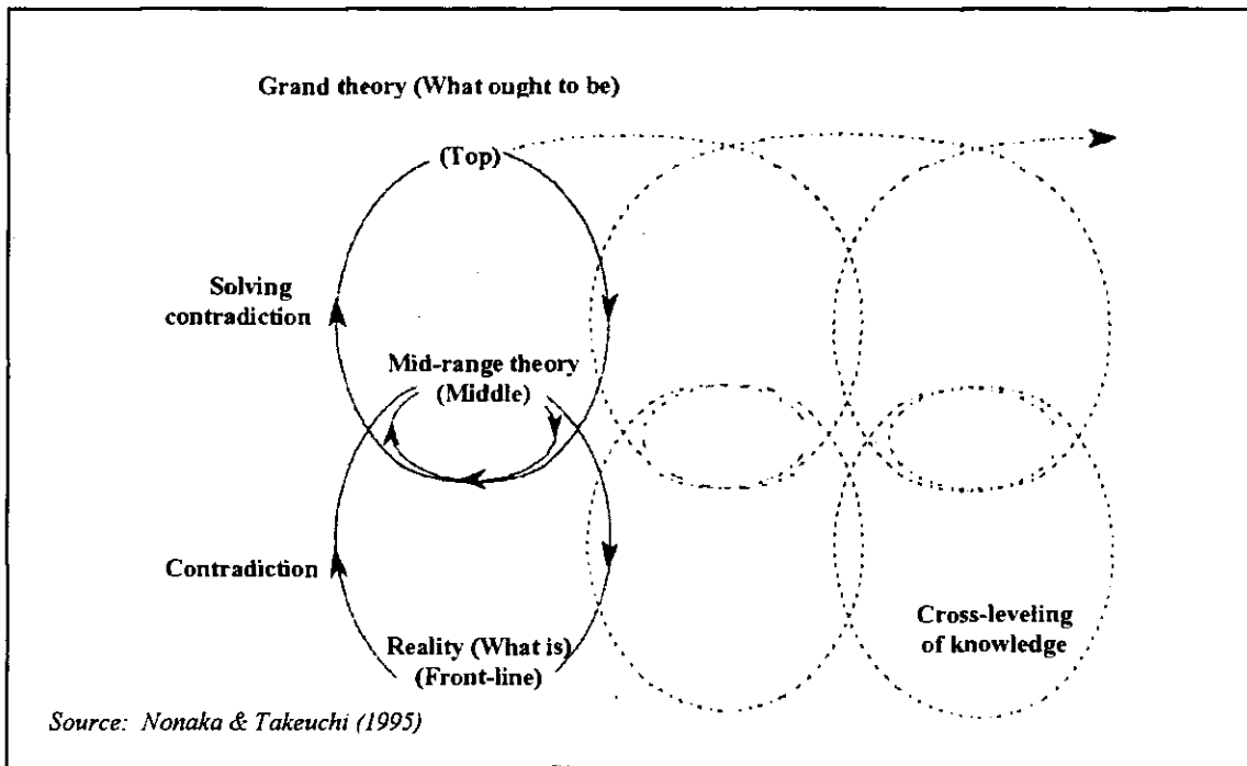
Figure 5.5 Middle-up-down Model
