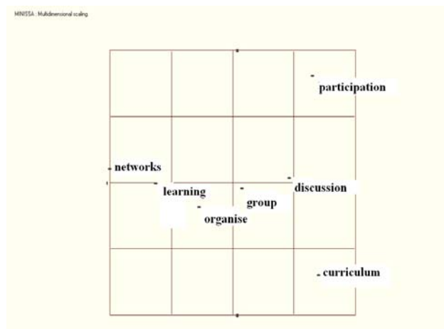
Diagram 1: Output of the two-dimensional scaling
