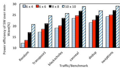
Fig. 14. Average network power efficiency.
