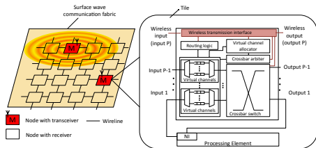
Fig. 2. Hybrid wireline-surface wave NoC architecture
