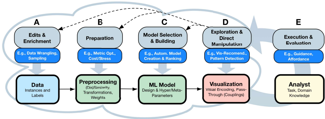
Figure 3: Proposed conceptual framework: A reference interactive VA/ML pipeline is shown on the left (A–D), complemented by several interaction options (light blue boxes) and exemplary automated methods to support interaction (dark blue boxes). Interactions derive changes to be observed, interpreted, validated, and refined by the analyst (E). Visual interfaces (D) are the “lens” between ML models and the analyst. Dashed arrows indicate where direct interactions with visualizations must be translated to ML pipeline adaptations. The colors of the pipeline components refer to the ones defined in the VA process model [1] shown in Figure 1.
