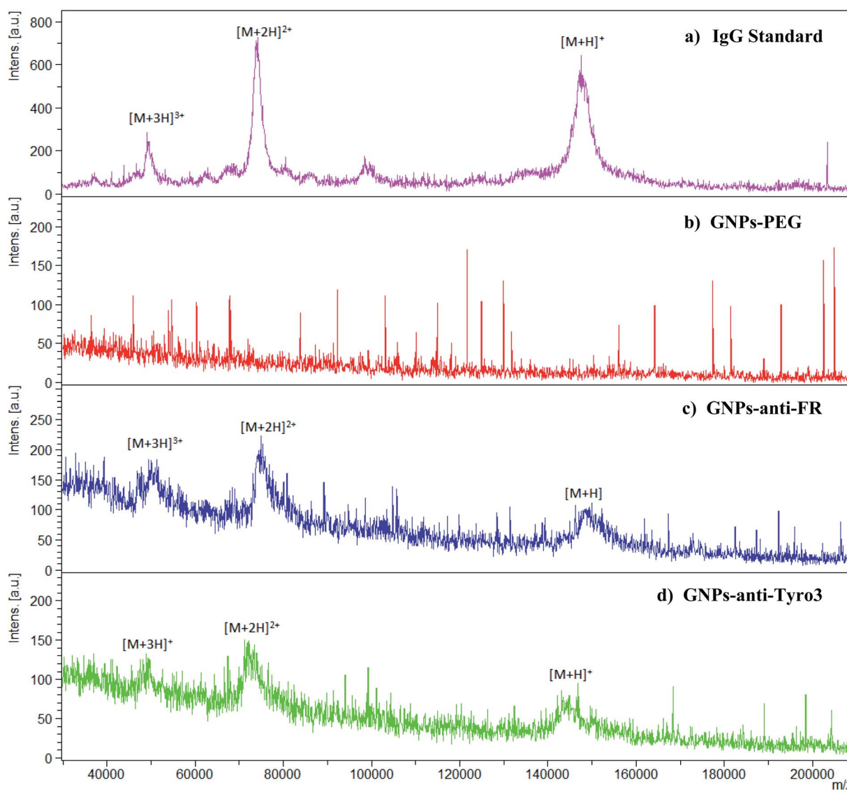
Fig. 6 MALDI-TOF spectra for (a) IgG as the standard, (b) GNPs-PEG, (c) GNPs-anti-FR and (d) GNPs-anti-Tyro3 are shown. High intensity peaks for IgG [M + H]^+ = m/z 148 286, [M + 2H]^{2+} = 74 478 and [M + 3H]^{3+} are seen. Spectra in (c) and (d) show the same peaks, however, they are absent in GNPs-PEG.
