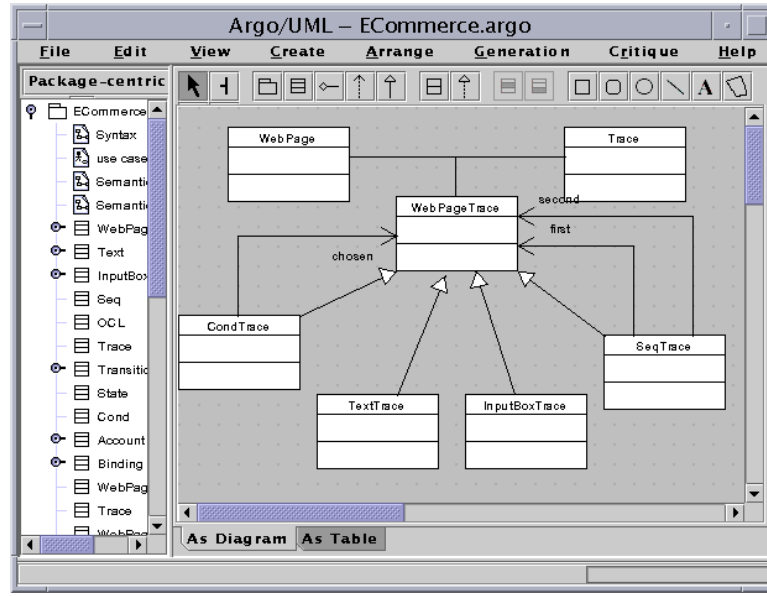
Figure 6: Semantic Mapping for ECommerce Profile
