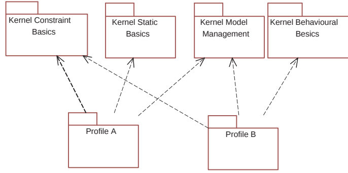
Figure 1: Profile architecture
