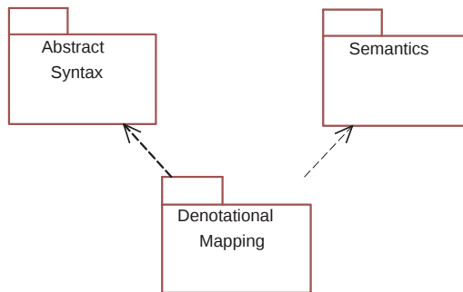
Figure 2: Profile semantics
