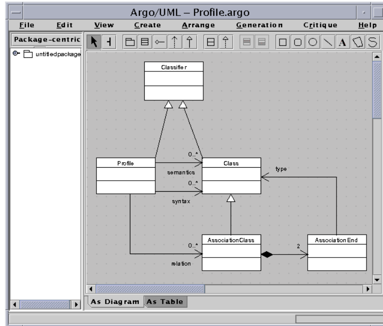
Figure 3: Meta Model for Profile
