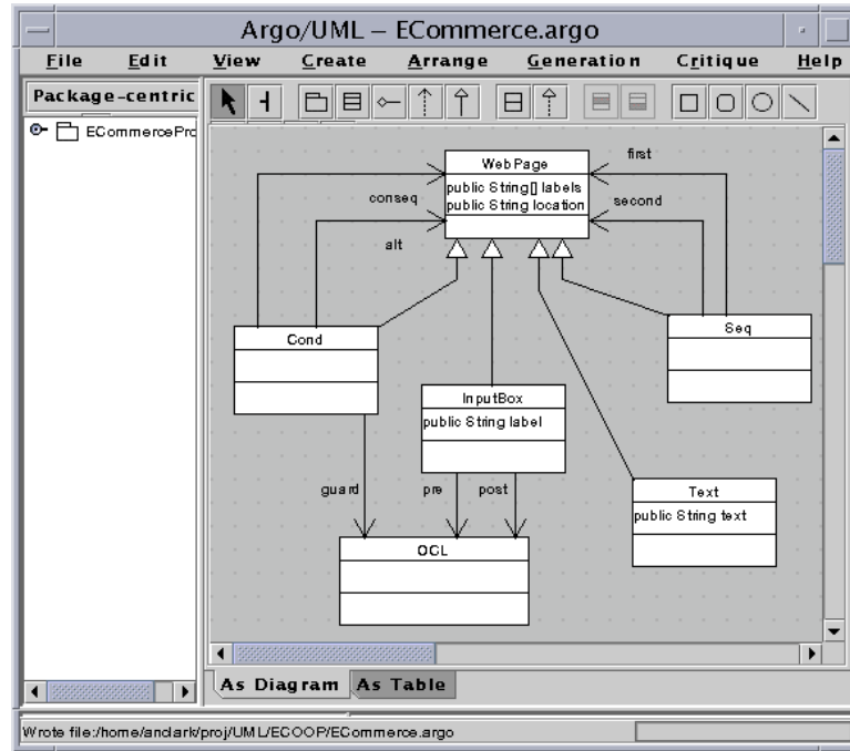
Figure 4: Syntax for ECommerce Profile
