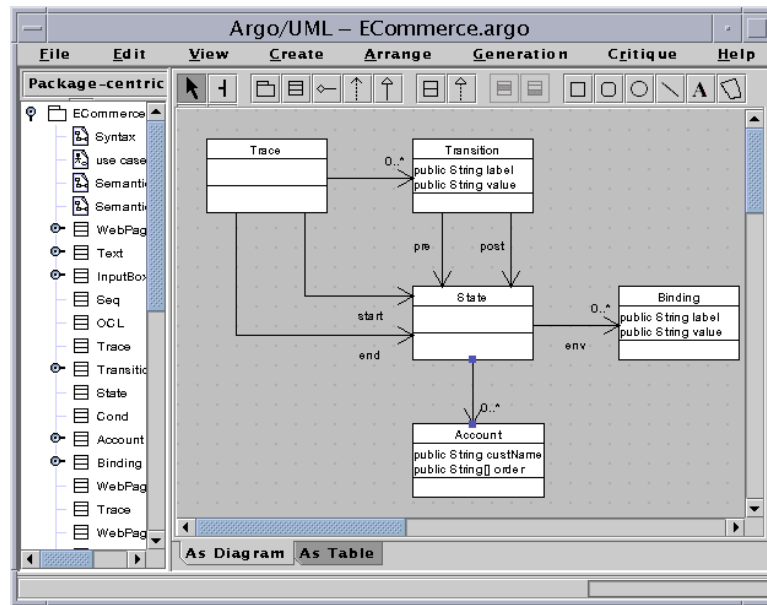
Figure 5: Semantics for ECommerce Profile
