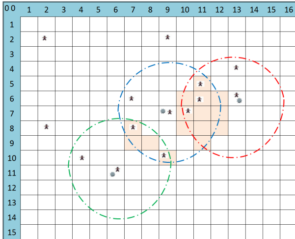
Fig. 8: Example of an overlap region in which some robots are in the wireless ranges of different coordinator robots and thus they must decide towards which target to move, according to a bio-inspired strategy.
