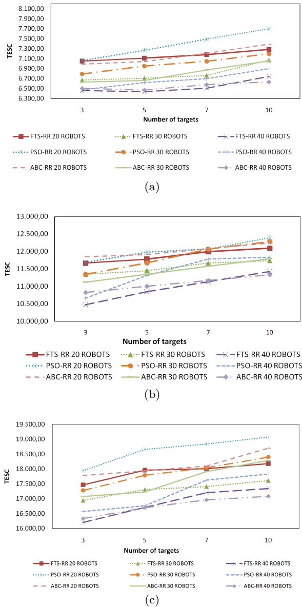
Fig. 11: Evaluation of Total-Energy-System- Consumed (TESC) for performing 3,5,7,10 targets and 3 robots needed to perform a target (a) 40x40 grid (b) 50x50 (c) 60x60.
