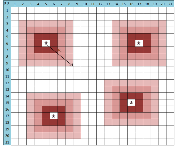
Fig. 7: Example of pheromone diffusion. When a robot moves to the new cell, it spreads the pheromone within a certain distance R_s . The intensity of pheromone decays according to the distance from the cell.
