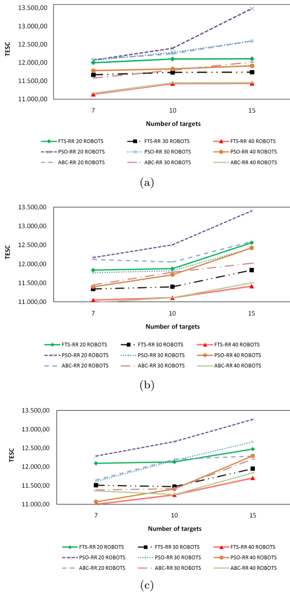
Fig. 12: Evaluation of Total-Energy-System-Consumed (TESC) for performing 7, 10, 15 targets and 3 robots needed to perform a target in 50x50 grid area (a) R_t = 6 (b) R_t = 8 (c) R_t = 10 .
