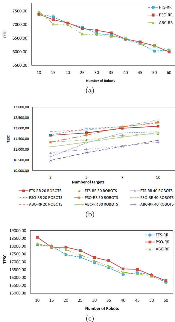
Fig. 10: Average-Energy-System- Consumed (TESC) evaluation for performing 3 targets and 3 robots needed to deal with a target (a) 40x40 grid (b) 50x50 (c) 60x60.
