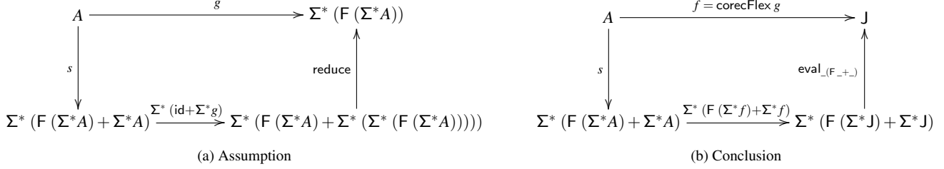
Figure 5: Mixed fixpoint
