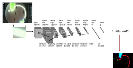
Figure 3. Caffe classification model while applying 32×32 patches.
