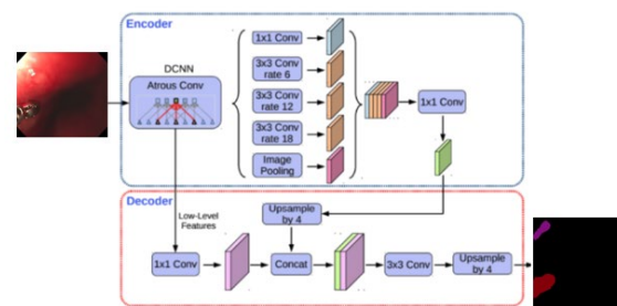
Figure 2. Segmentation applying deepLabV3 model.
