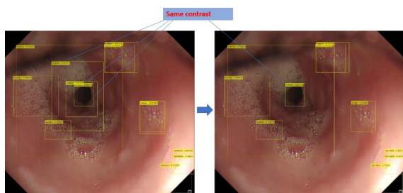
Figure 7. The impact of thresholding of model of fast-running-nas. Left: threshold=0.1; right threshold=0.3.
