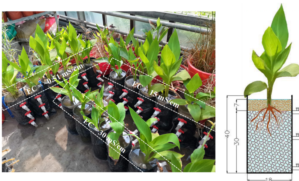
Fig. 1. A photo and schematic diagram of CW microcosms (Unit: centimeter). EC: electrical conductivity.
