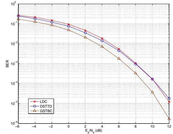
Fig. 9. BER performance comparison with the linear dispersion and DSTTD codes (both with code rate of 2) for K = 4 , N = 4 and throughput of 6 bits/s/Hz.
