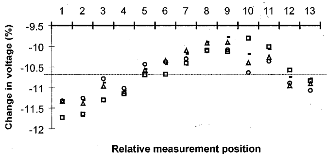
Fig. 3. Mean change in voltage versus measurement position on the saline tank, for dilution by 10%, for each of the four optimization techniques, 1a = triangle, 1b = dash, 2a = square, and 2b = circle. The dotted straight line shows the expected change of voltage of 10.7%.
