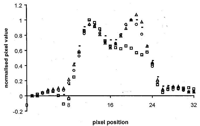
Fig. 4. Example of averaged cross-sectional profile through the images of the two sponges separated by 5.6 cm in the saline-filled tank for the four techniques; 1a = triangle, 1b = dash, 2a = square and 2b = circle.
