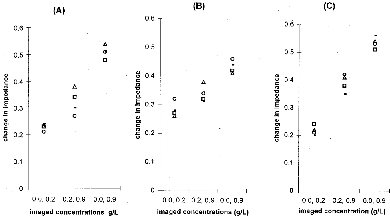
Fig. 7. Comparison of impedance change against saline concentration for each of the three volunteers and the four optimization techniques; 1a = triangle, 1b = dash, 2a = square and 2b = circle.
