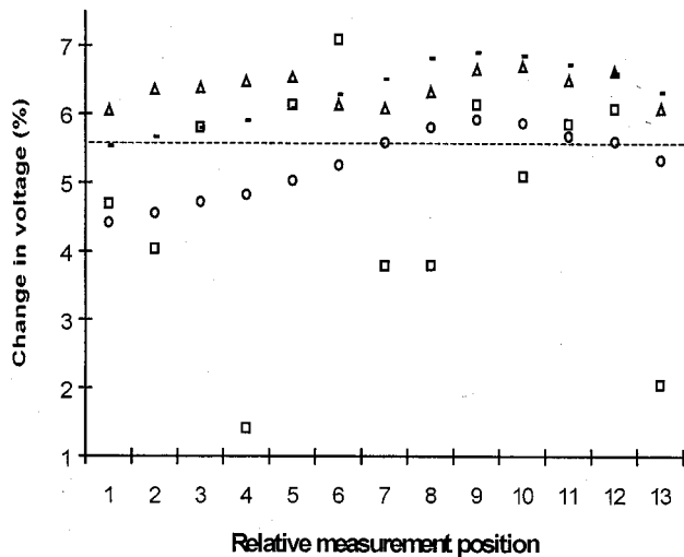
Fig. 2. Graph of the change in voltage versus measurement position on the Cardiff Cole phantom for each of the four optimization techniques, 1a = triangle, 1b = dash, 2a = square, and 2b = circle. The dotted straight line shows the expected change of voltage due to introduction of additional resistance.
