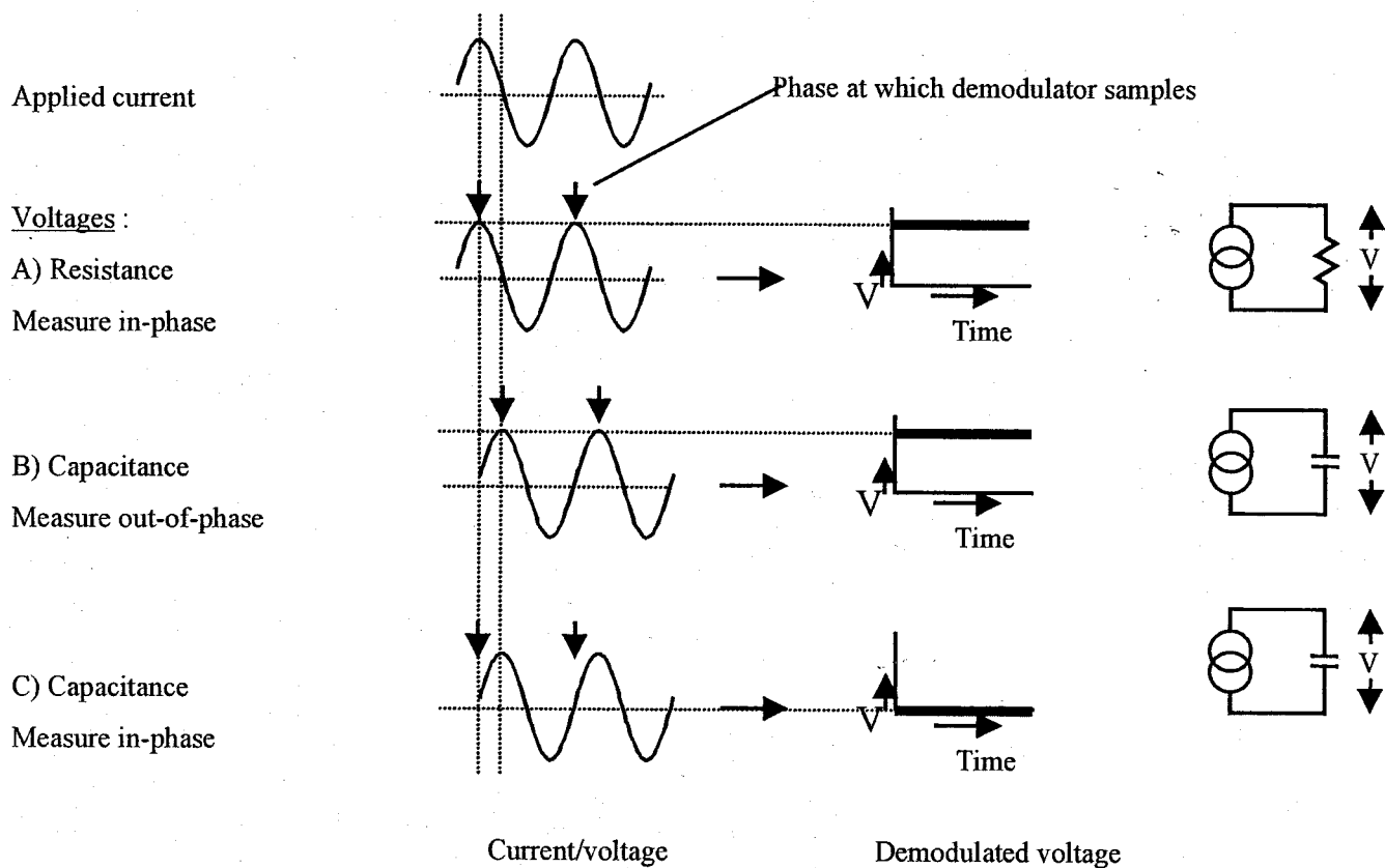
Fig. 1. Demodulation. The voltage that results from an applied current is in phase for a resistor (A) and 90^\circ out of phase for a capacitor (B&C). The in or out of phase components may be selected by setting the phase at which the demodulator measures. The effects of capacitance may be ignored by setting the demodulator to measure at in-phase; it will then only transmit the resistive component of a signal.
