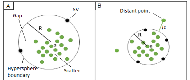
Figure 1. SVDD hypersphere
