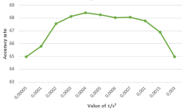
Figure 3. Accuracy of the Gaussian kernel SVDD w.r.t. 1/s^2
