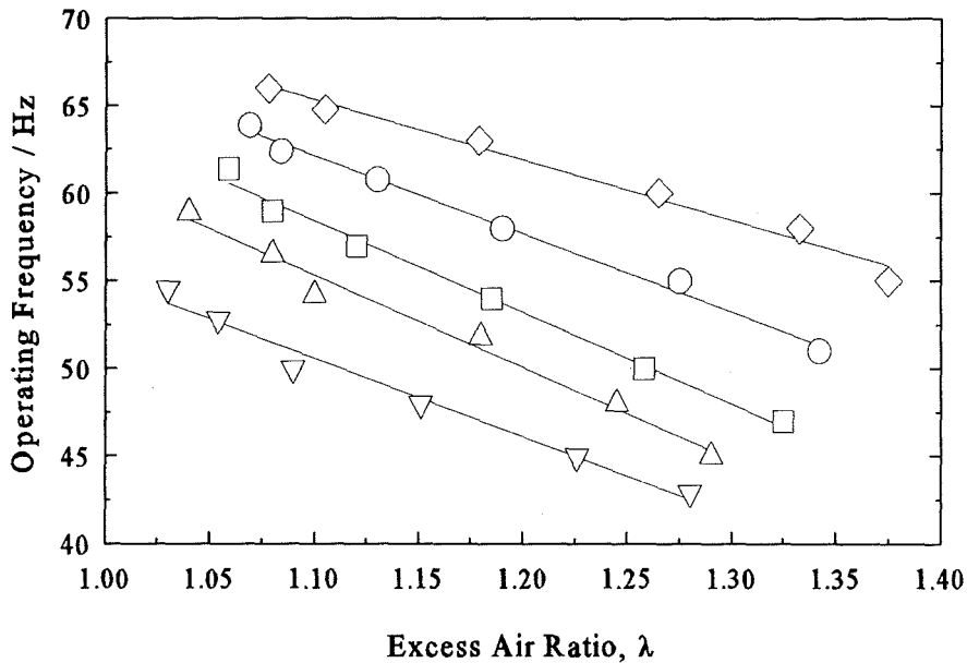
Fig. 4.10 Operating frequency vs \lambda for the 15 kW combustor at fixed tailpipe length and flapper valve thickness. Symbols as in Fig. 4.9.
