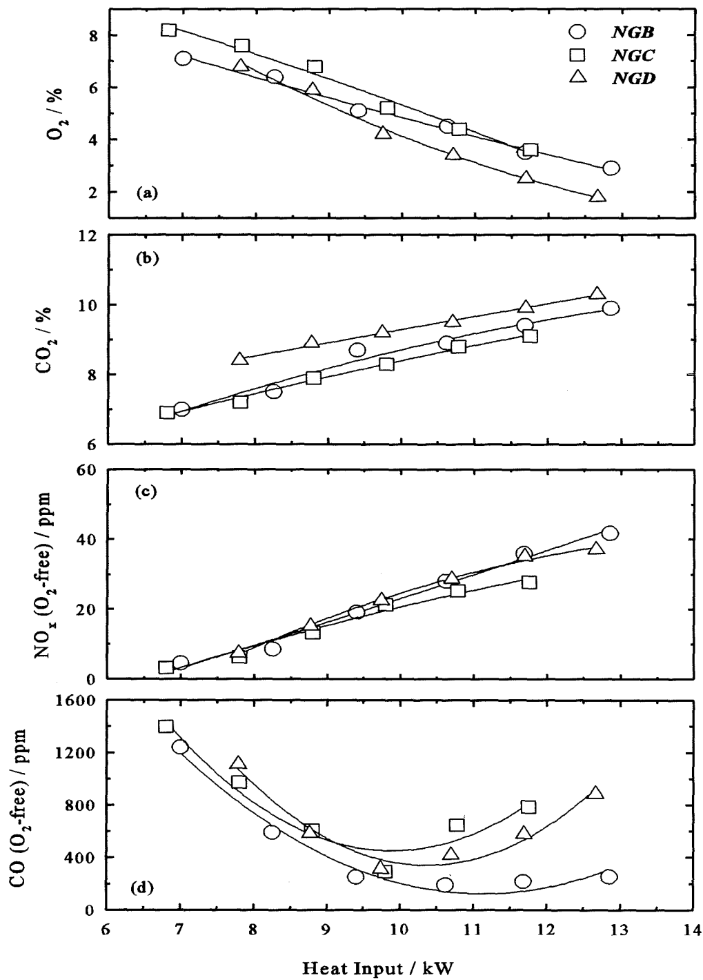
Fig. 6.45 Variation of concentrations of combustion products a) O_2 , b) CO_2 , c) NO_x and d) CO concentrations with heat input burning test gases NGB, NGC and NGD. Configuration: combustion chamber volume 360 ml, tailpipe length 2500 mm and flapper valve thickness 0.15 mm.
