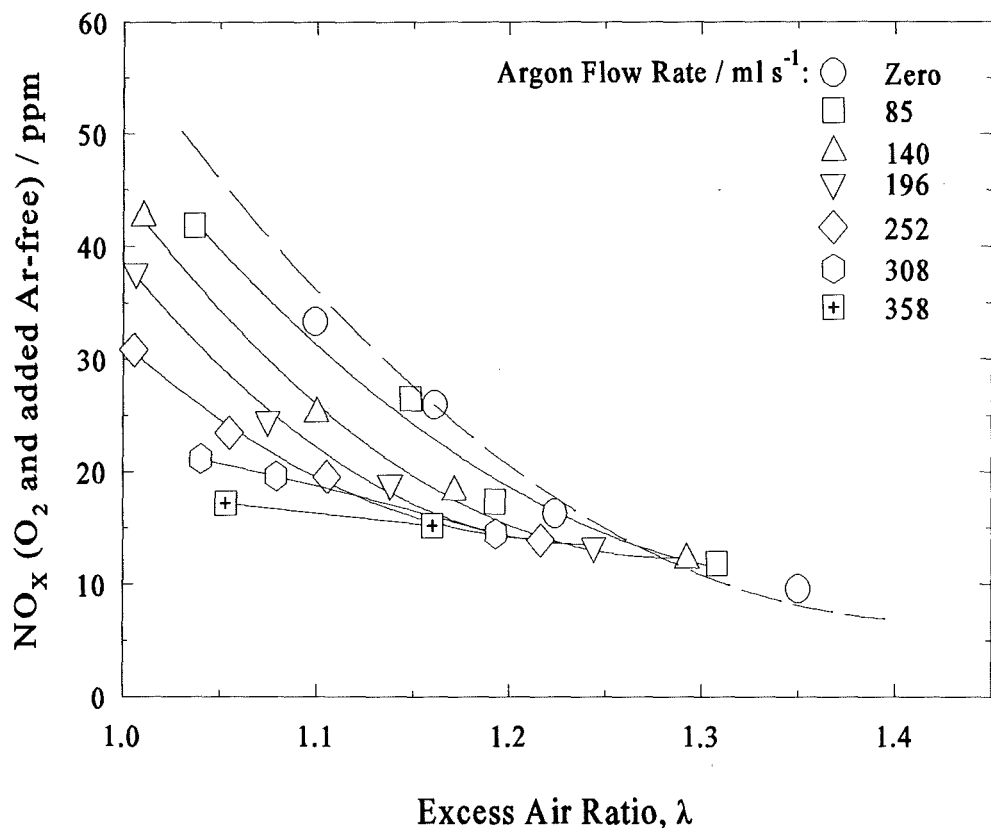
Fig. 6.26 Variation of \text{NO}_x corrected to zero oxygen and added argon with \lambda at various rates of Ar injection. The broken line represents the \text{NO}_x vs \lambda at various operating condition of the 15 kW combustor with zero argon injection. Configuration used here: combustion chamber volume of 370 ml, tailpipe length of 1500 mm and flapper valve thickness 0.13 mm.
