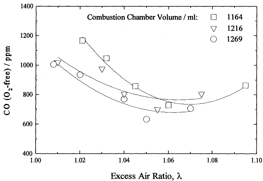
Fig. 6.34 Variation of CO with \lambda for the nominally 30 kW combustor, using fixed tailpipe length of 2000 mm and the specified combustion chamber volumes.
