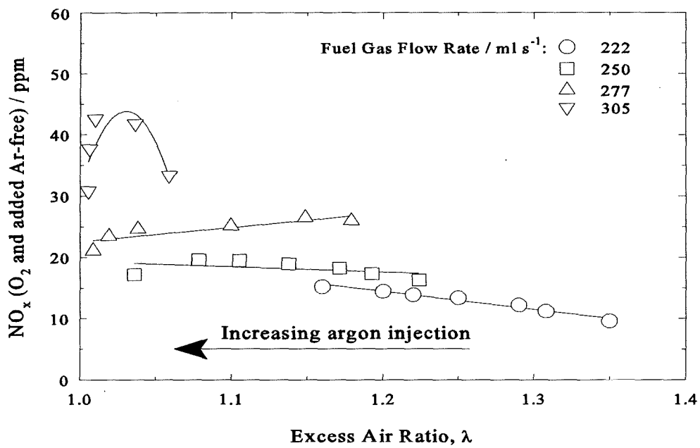
Fig. 6.27 \text{NO}_x vs argon excess air ratio, \lambda at various gas input rates. Data and configuration as in Fig. 6.26.
