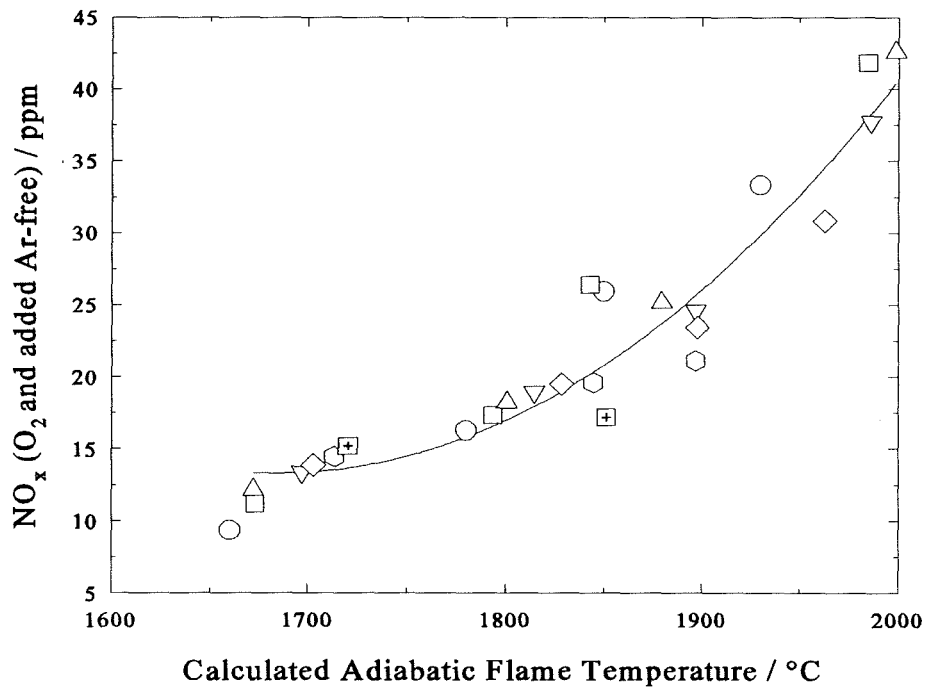
Fig. 6.30 Variation of \text{NO}_x (corrected to zero oxygen and added argon) as a function of calculated adiabatic flame temperature at various rates of argon from zero to 350 \text{ ml s}^{-1} . Configuration and symbols as in Fig. 6.26.
