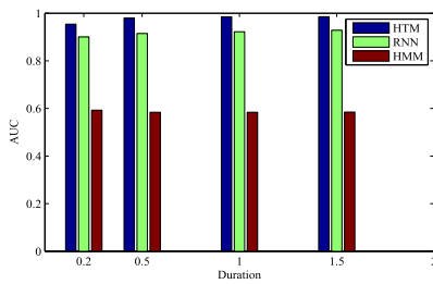
FIGURE 3. AUC score for data sequence field modification case.
