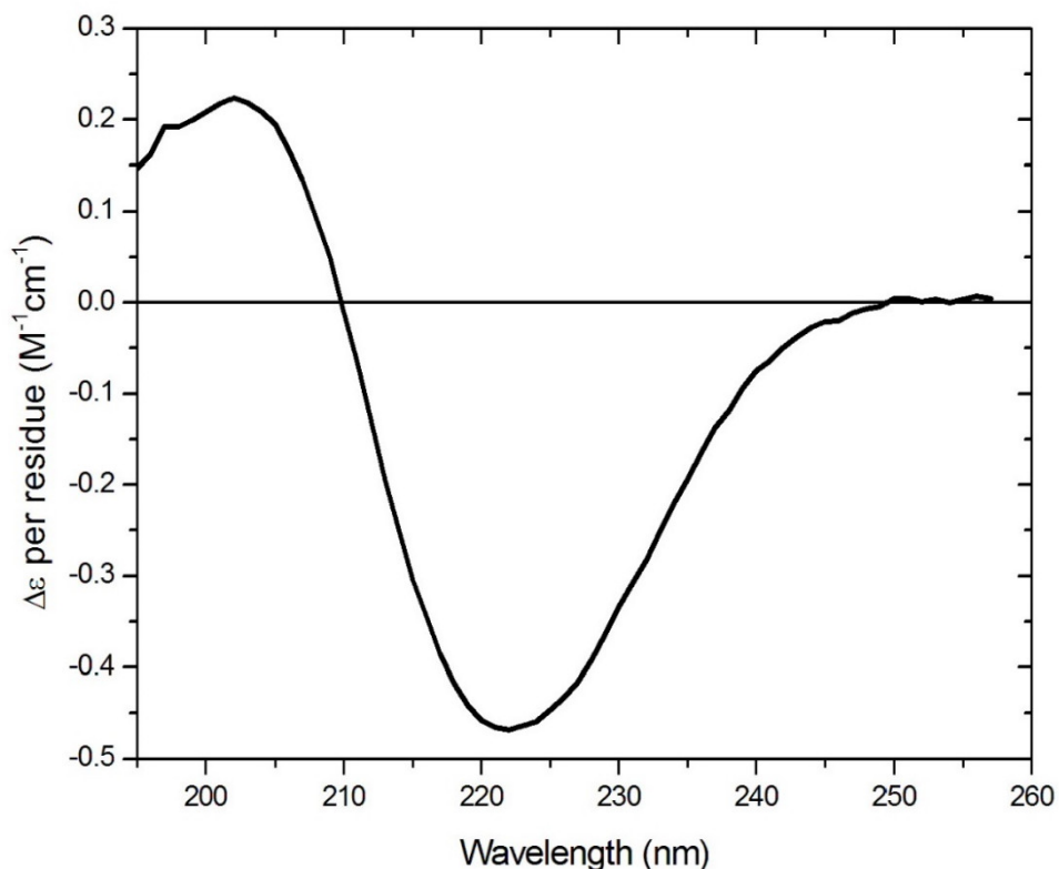
Figure 2. The far UV circular dichroism spectrum of a Lexicon cyclic peptide with the structure cyclo(sRC(C8)FsSrc(C8)fS), where L and D forms are represented by upper- and lower-case letters, respectively. The data are expressed as Molecular Circular Dichroism, or \Delta\epsilon per residue, using a mean molecular weight of 149. The single negative CD minimum at \sim 222 nm with the crossover at 210 nm is representative of the signature of a \beta -turn/ \beta -turn structure [8,9].
