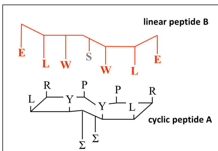
Figure 4. Sequence structure of the cyclic peptide aptamer (A) and linear peptide (B) employed in this study.
