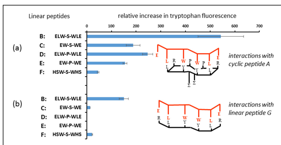
Figure 6. (a) Fluorescence enhancement observed as a result of incubating cyclic peptide A at 37 °C with the linear peptides shown. (b) Fluorescence enhancement observed as a result of incubating linear peptide G at 37 °C with the linear peptides shown. Tryptophan fluorescence is shown here, since tryptophan is the common feature across the whole series of linear peptides containing tryptophan, and these results are mirrored by the tyrosine readings obtained (data not shown).
