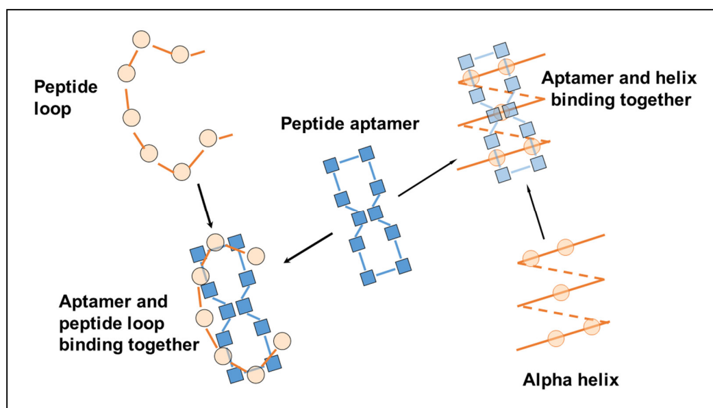
Figure 3. Peptide aptamers are a close fit with common structures in proteins.
