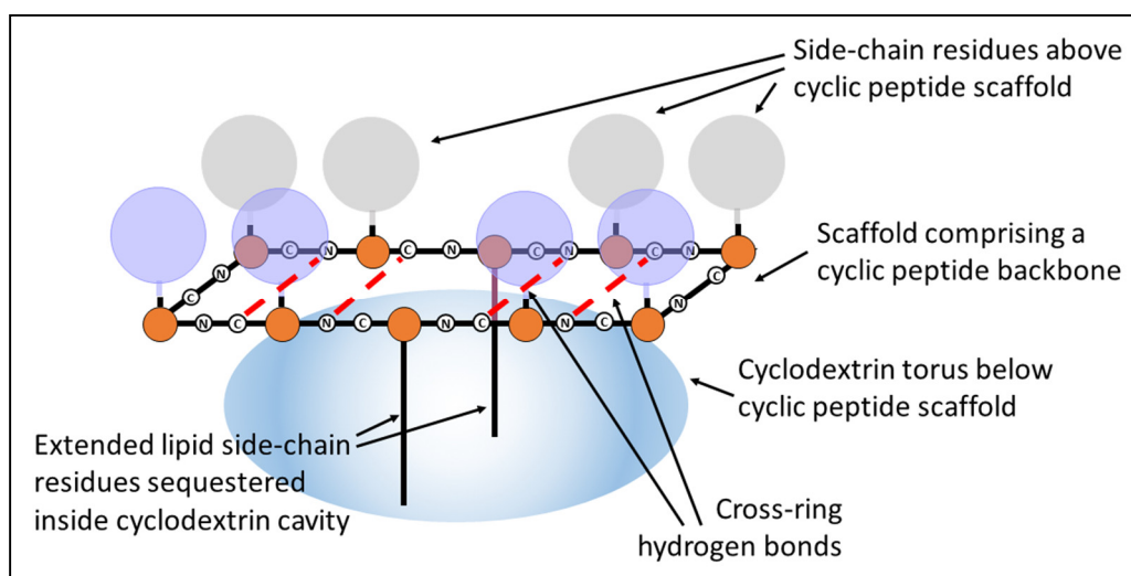
Figure 1. Structure and configuration of a peptide aptamer.
