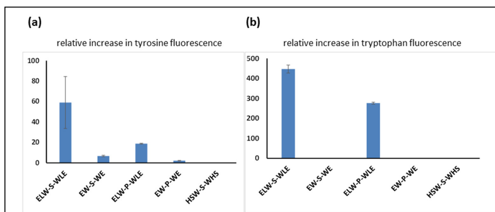
Figure 5. (a) Tyrosine fluorescence enhancement observed as a result of incubating cyclic peptide A at room temperature with the linear peptides shown. (b) Tryptophan fluorescence enhancement observed as a result of incubating cyclic peptide A at room temperature with the linear peptides shown.
