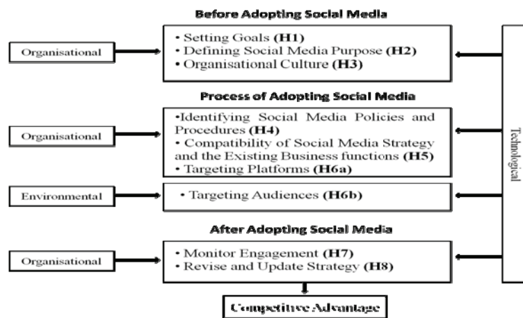
Figure 1. BPA framework
