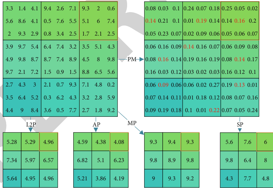
FIGURE 3: Comparison of four different pooling techniques (red rectangle indicates the example discussed in Section 3.2).
