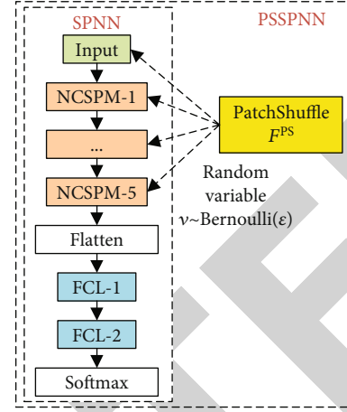
FIGURE 7: Build PSSPNN from SPNN.
