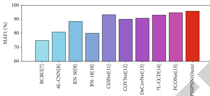
FIGURE 12: Algorithm comparison in terms of MA F1.
