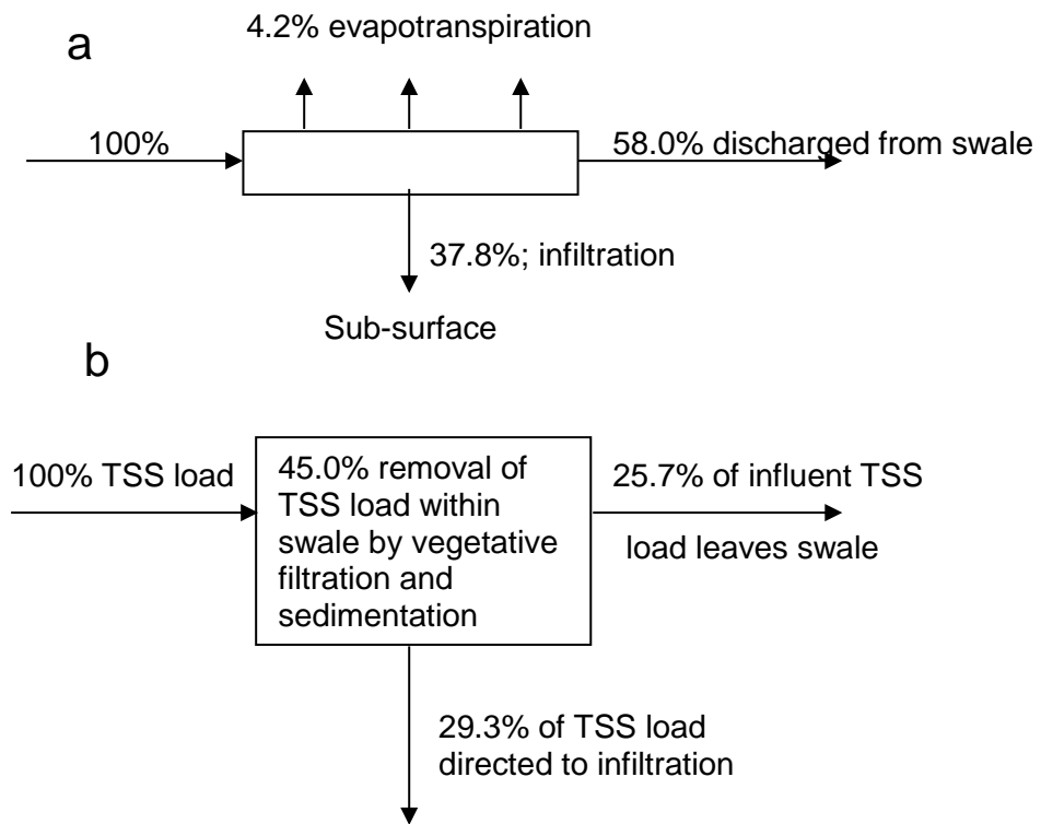
Figure S1. a) Diagrammatic representation of typical mean flow distributions within a swale. b) Diagrammatic representation of typical mean TSS loads during removal within a swale.
