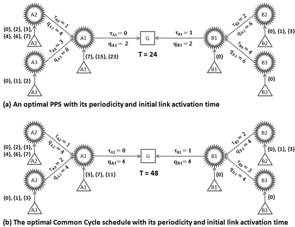
Fig. 7. An optimal PPS and an optimal Common Cycle schedule for Example 3.
