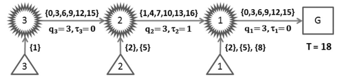
(c) The optimal Common Cycle schedule with link activation times
