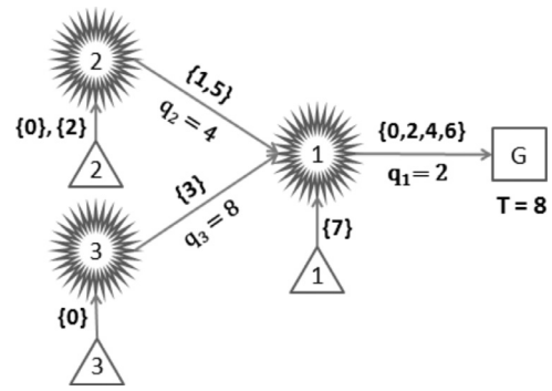
Fig. 4. An optimal PPS with q_1 = 2 for Example 2, specified by its link activation times.
