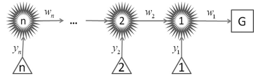
Fig. 1. A network with the chain structure.
