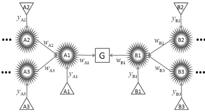
Fig. 6. The structure of a binary tree.
