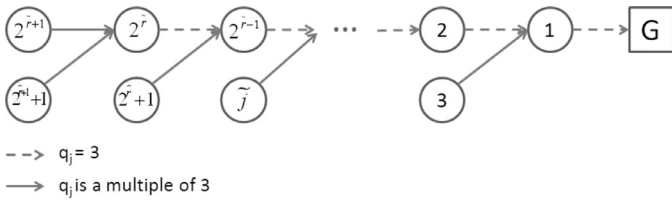
Fig. 5. Illustration of J_2 subnetwork part of a feasible solution with q_1 = 3 .
