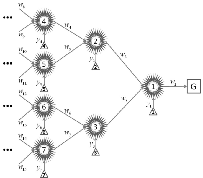
Fig. 3. The structure of a half binary tree.
