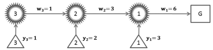
(a) An instance of the chain network with link data load
