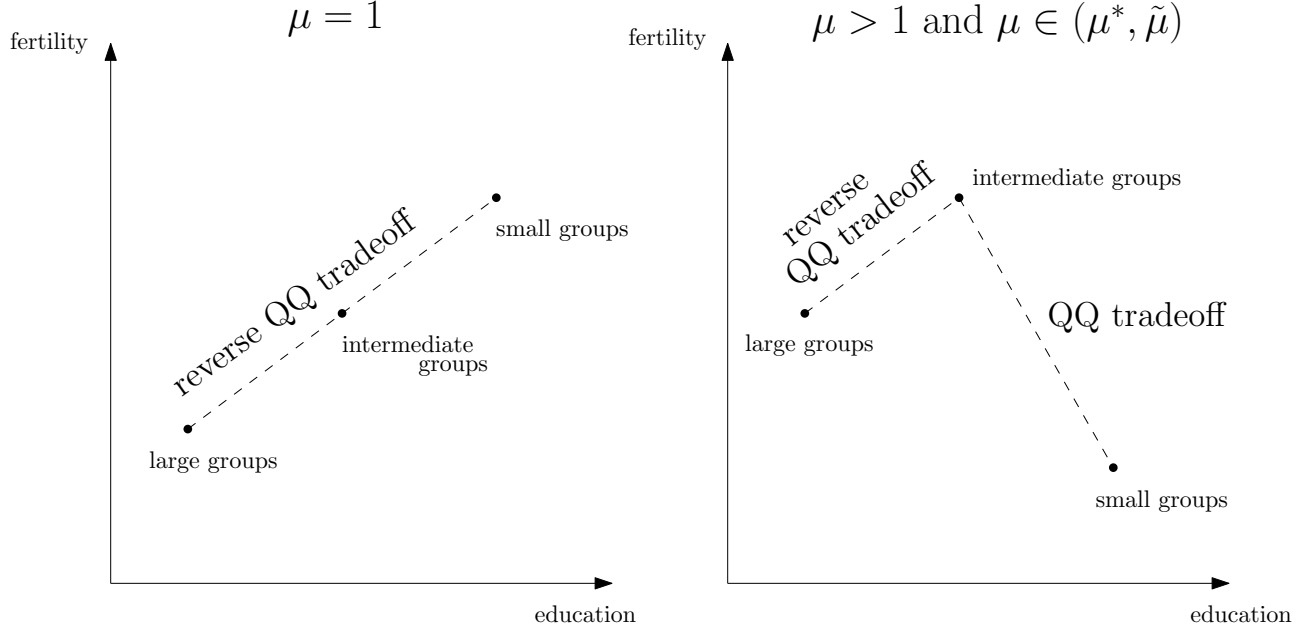
Figure 1: Propositions 2 (left panel) and 3 (right panel)
