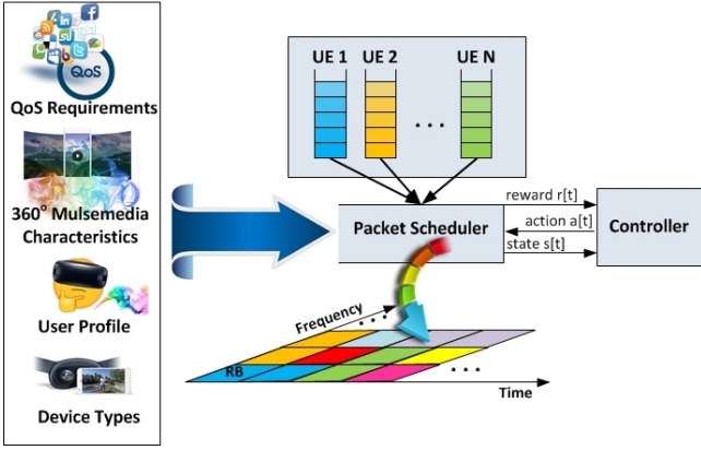
Fig. 3 Packet Scheduler Based on Proposed RL Framework. and unpredictable network conditions. In this situation, only some particular QoS objectives are addressed, and the overall QoS satisfaction is degraded. However, one way to overcome this major drawback is to propose a framework able to select according to the actual network conditions and 360° mulsemmedia traffic characteristics, the best scheduling rule in such a way that the overall QoS satisfaction is maximized. To make this solution tractable in real time scheduling systems, we propose a solution based on Reinforcement Learning which is able to learn the best rule to be applied based on the instant scheduler states.
