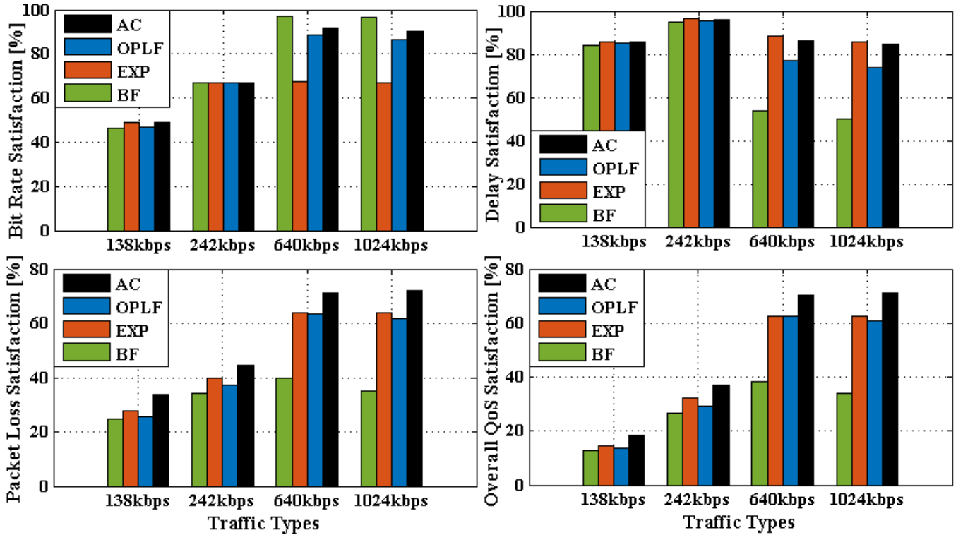
Fig. 4 Simulation Results based on RL AC Framework
