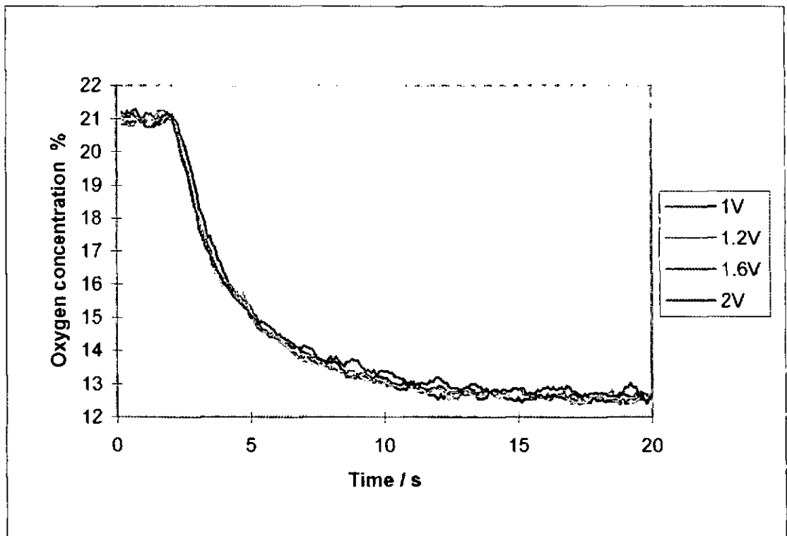
Figure 4.19 Concentration step using an amperometric sensor with pump voltage
