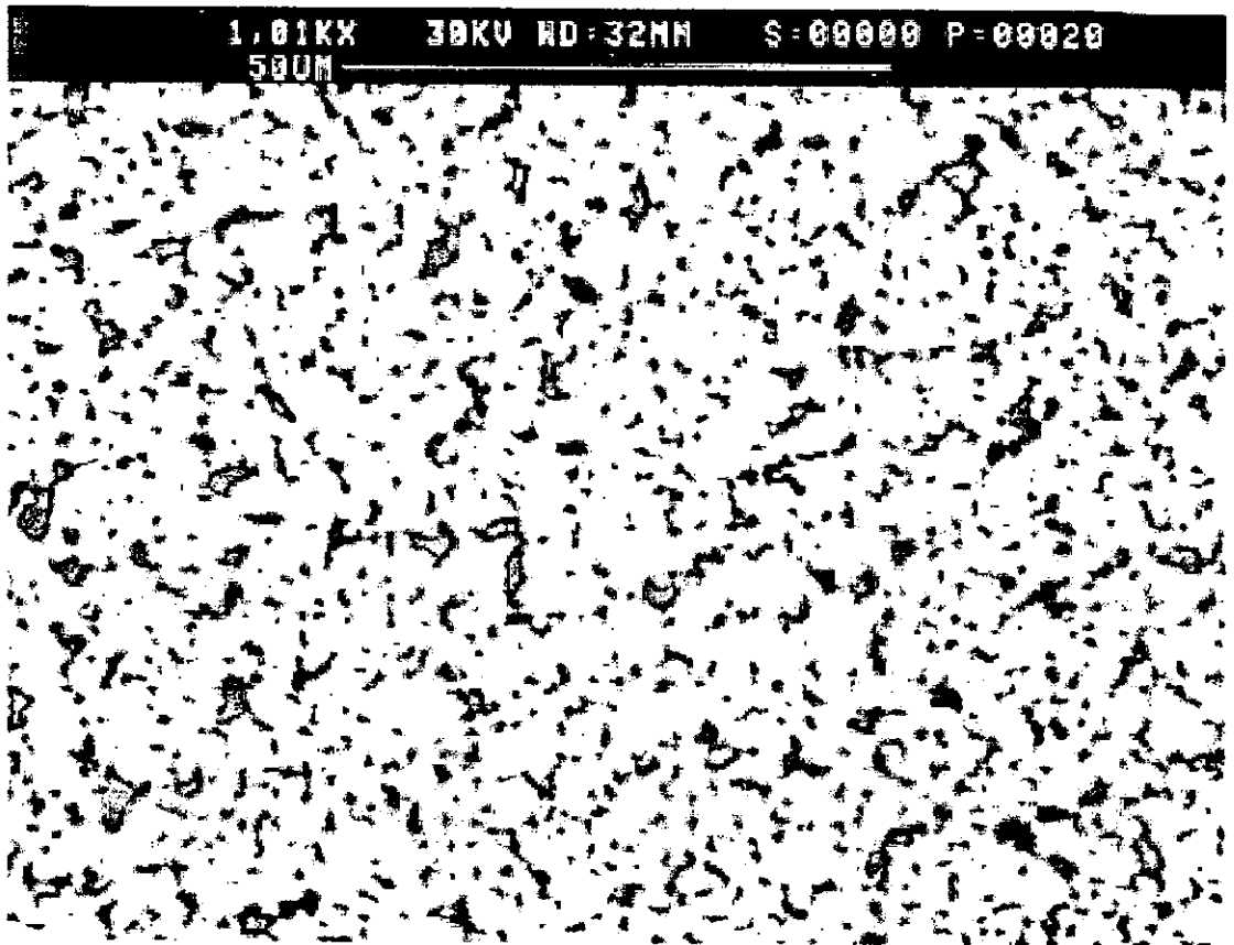
Figure 5.43 Platinum cermet electrode face fired at 1000°C
