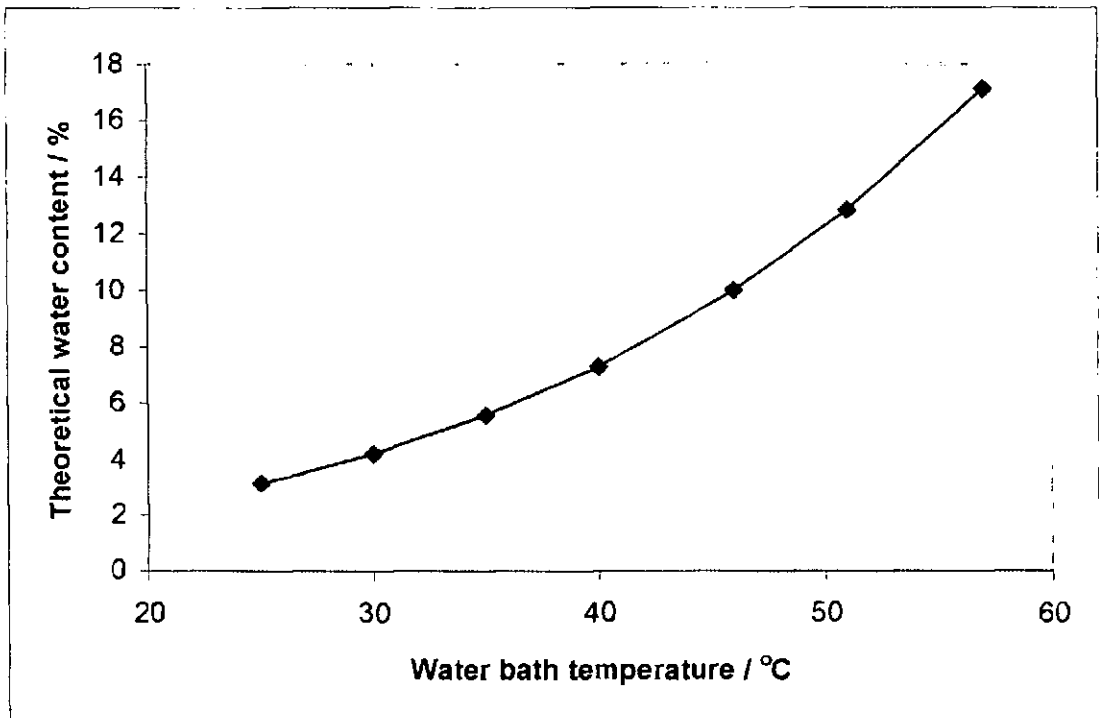
Figure F52 Translation of water bath temperature to percentage water content of gas
