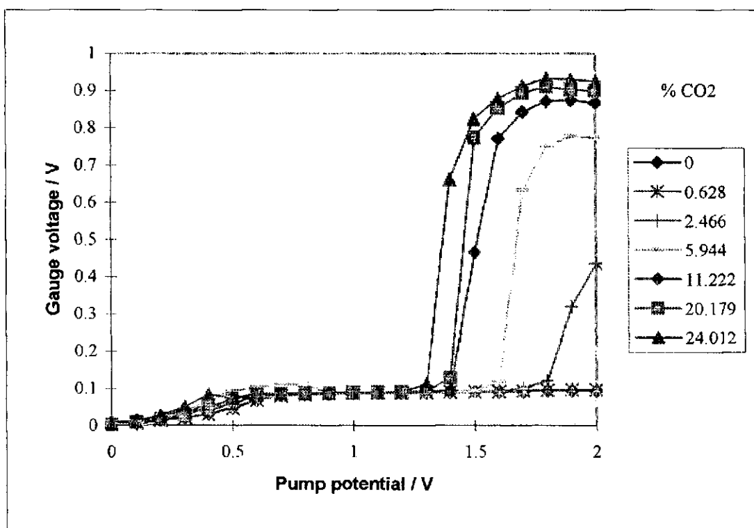
Figure F78 Gauge EMF behaviour with CO 2 variation
