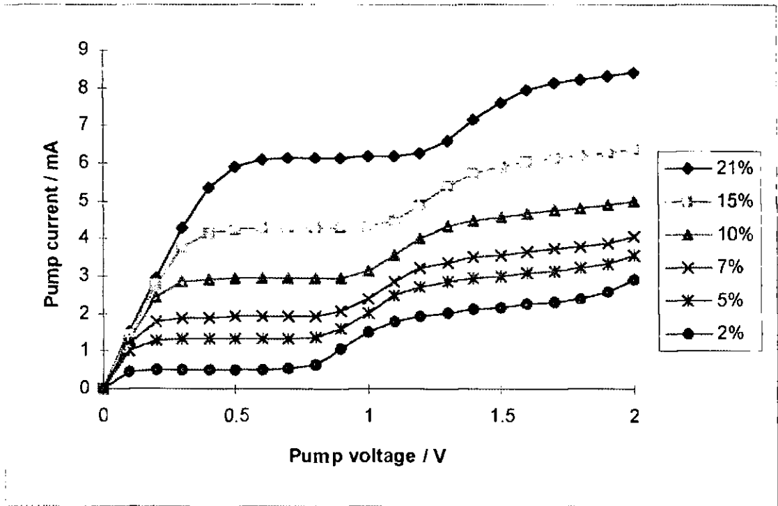
Figure F50 Pump current behaviour with oxygen variation in humid atmospheres
