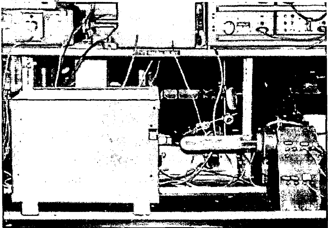
Figure C3 Sensor test-rig
