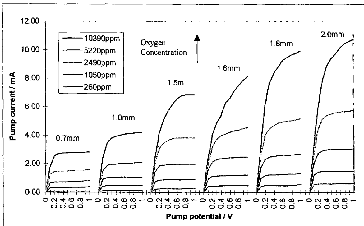
Figure F13 Current / voltage characteristics for sensors with large diameter diffusion barriers
