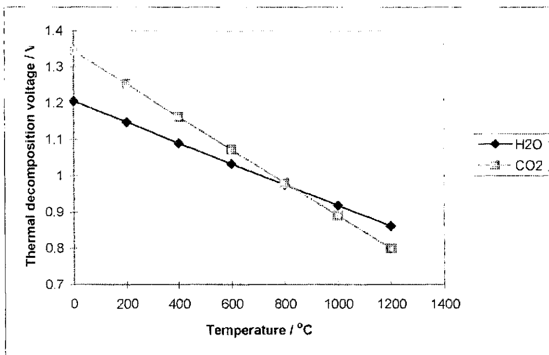
Figure F64 Comparison of temperature dependence of the thermal decomposition voltage for H 2 O and CO 2
