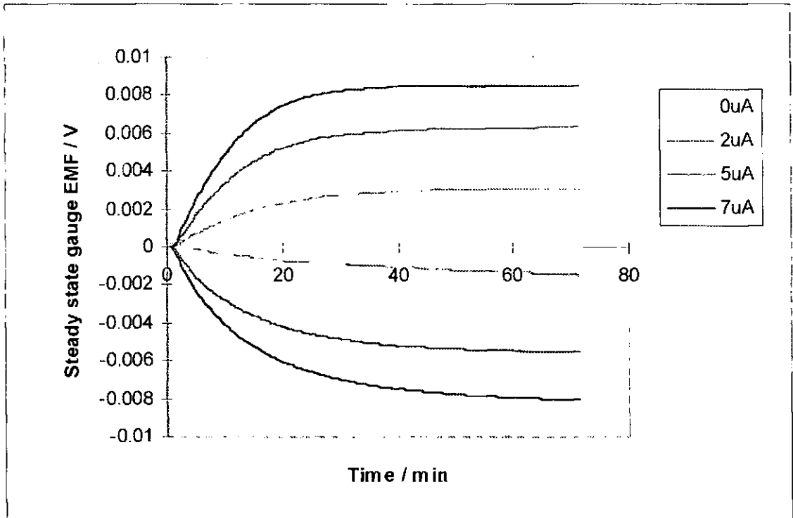
Figure F39 Steady state leakage test
