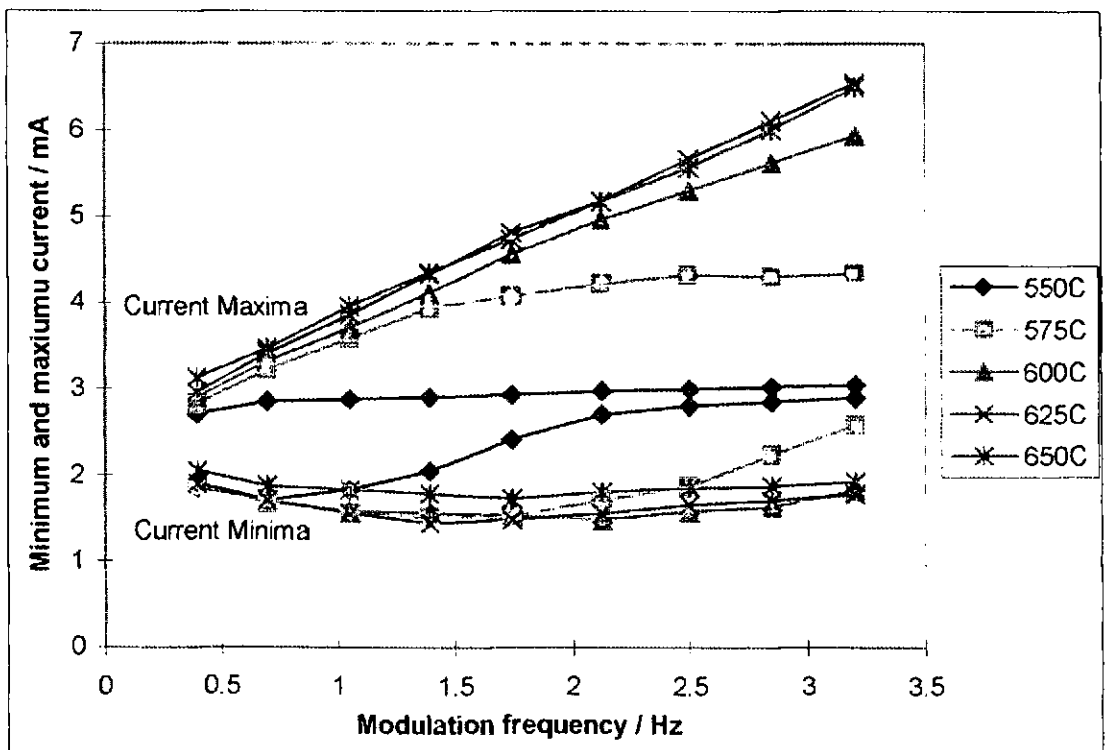
Figure 4.29 Modulation limits vs. frequency
