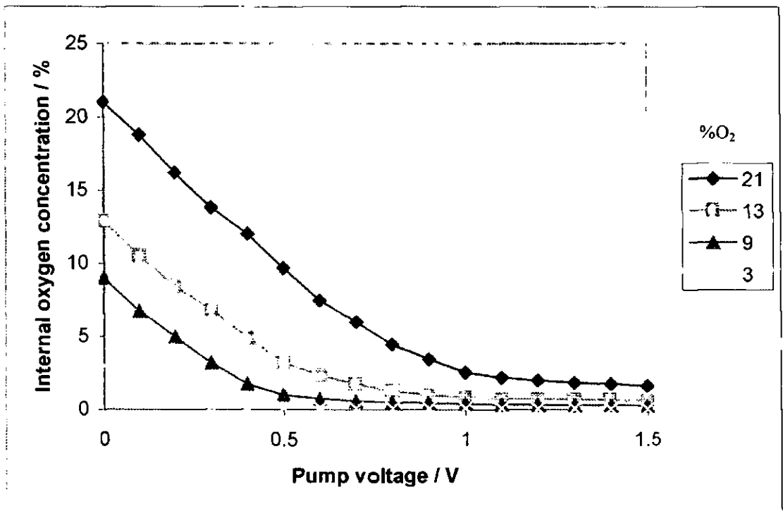
Figure F6 Calculated internal oxygen concentrations
