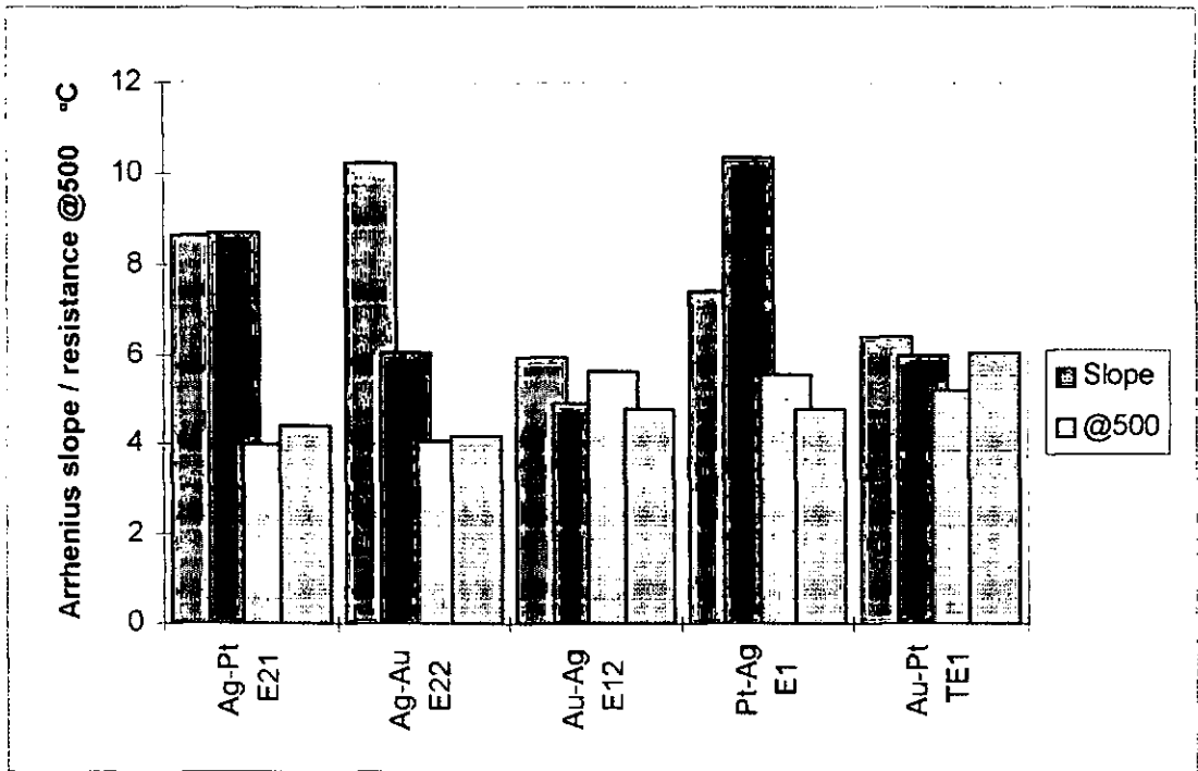
Figure 5.16 Bar chart of layered electrode Arrhenius parameters
