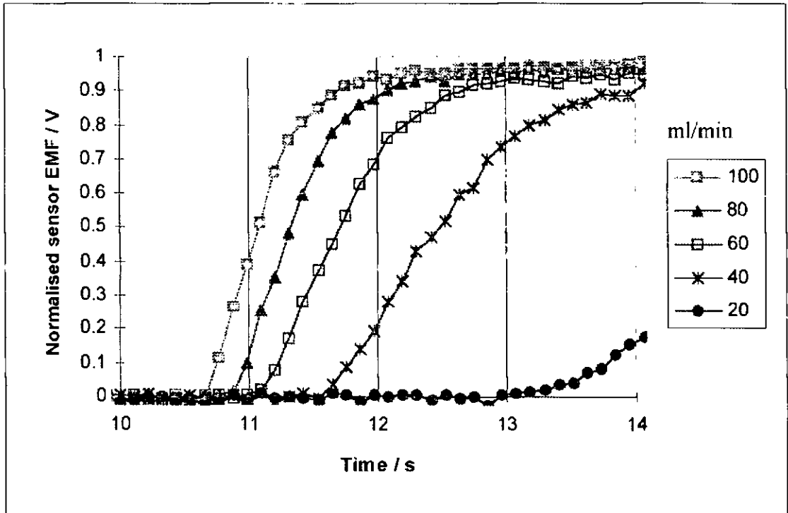
Figure 3.10 Enlarged step change response with flow rate variation
