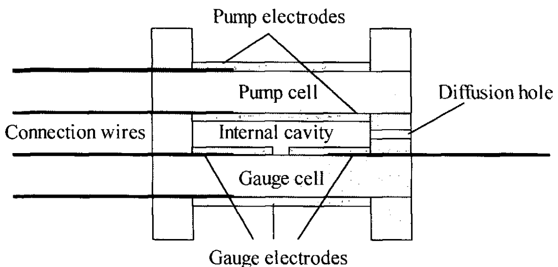
Figure 1.7 Split electrode amperometric sensor
