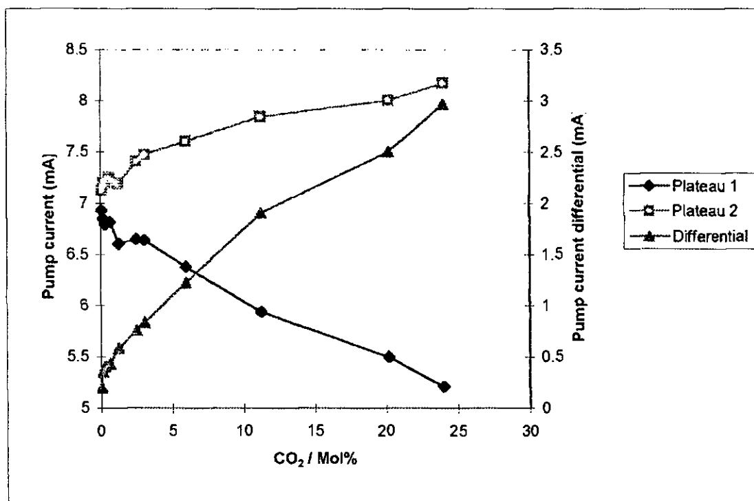
Figure F76 Pump current behaviour with CO 2 variation
