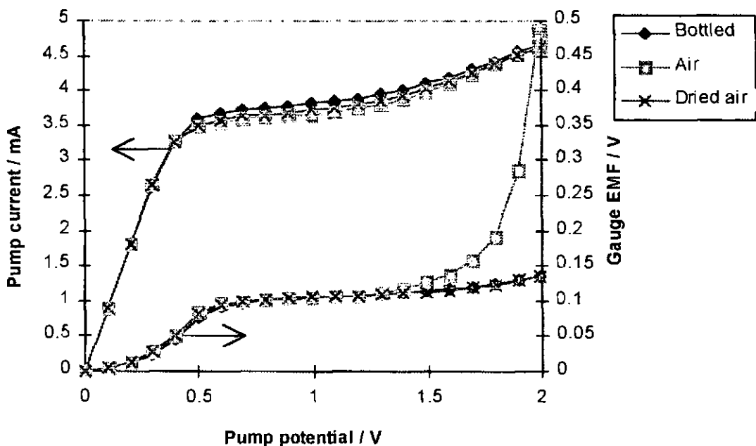
Figure F49 Sensor response to atmospheric, dried and bottled gases
