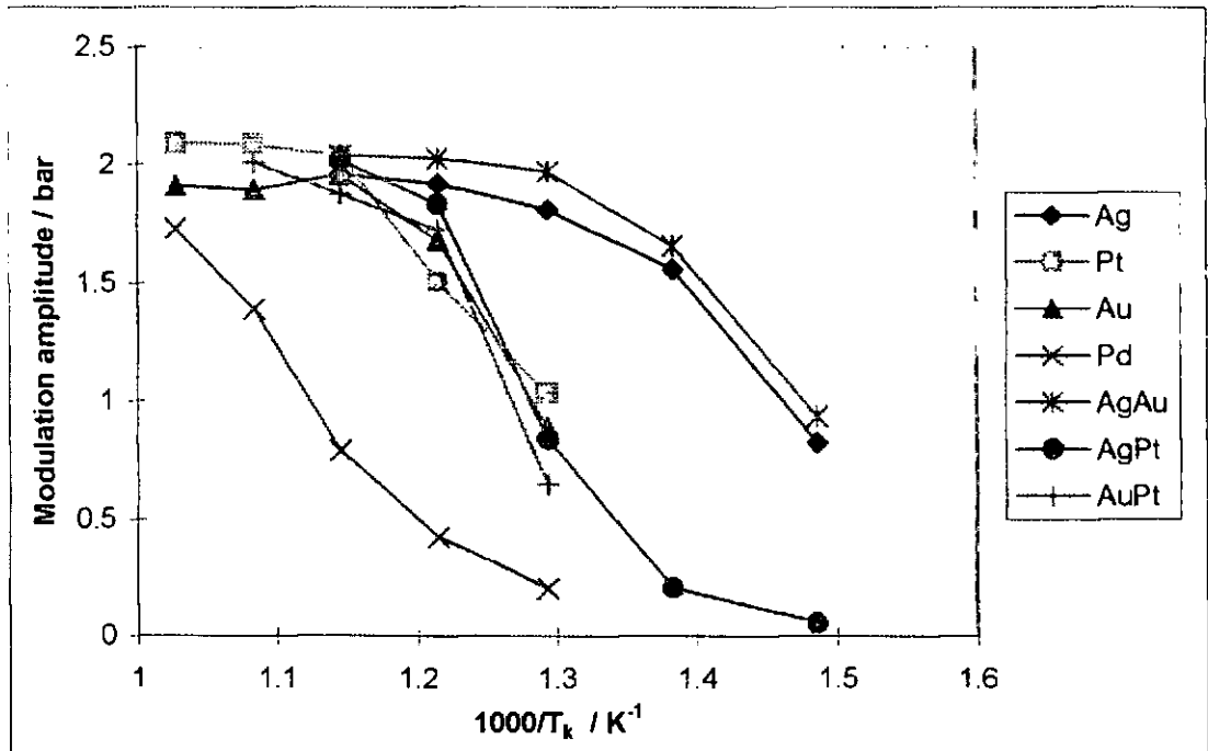
Figure 5.29 Modulation amplitude vs. temperature for various electrodes
