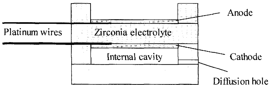
Figure 1.4 Two electrode amperometric sensor
