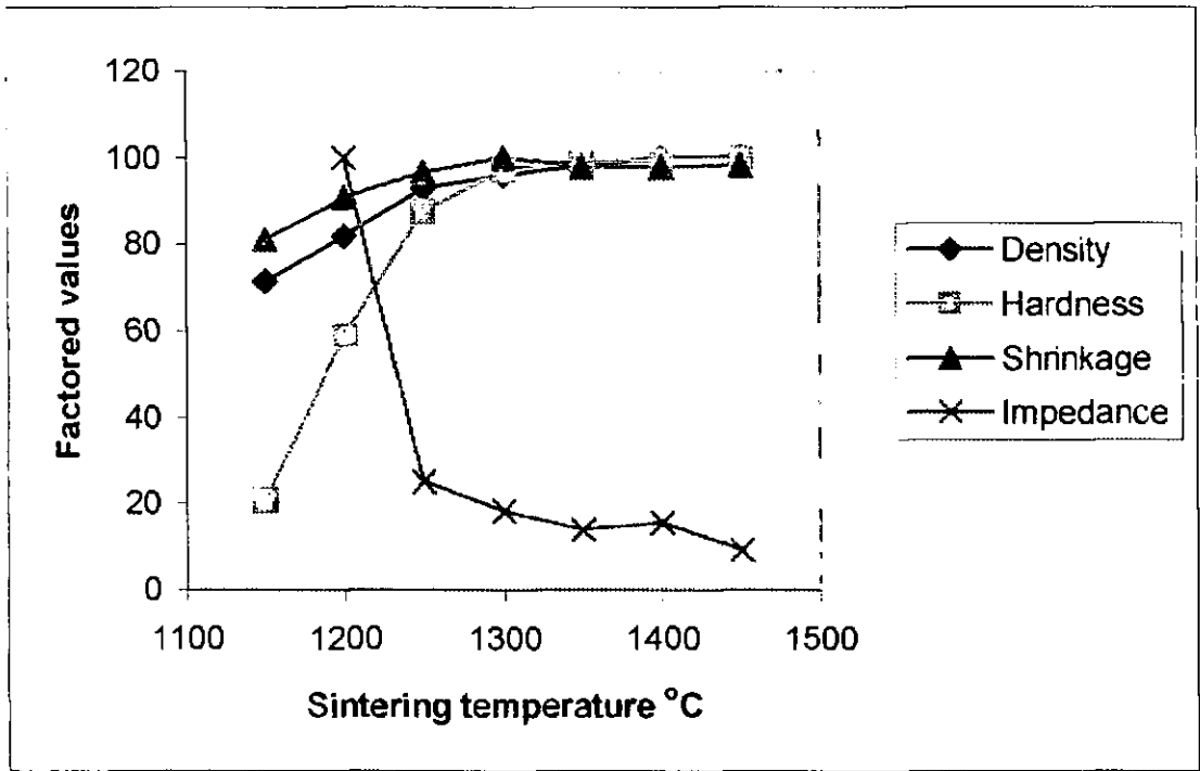
Figure 3.8c Sintering temperature effects on electrolyte properties.
