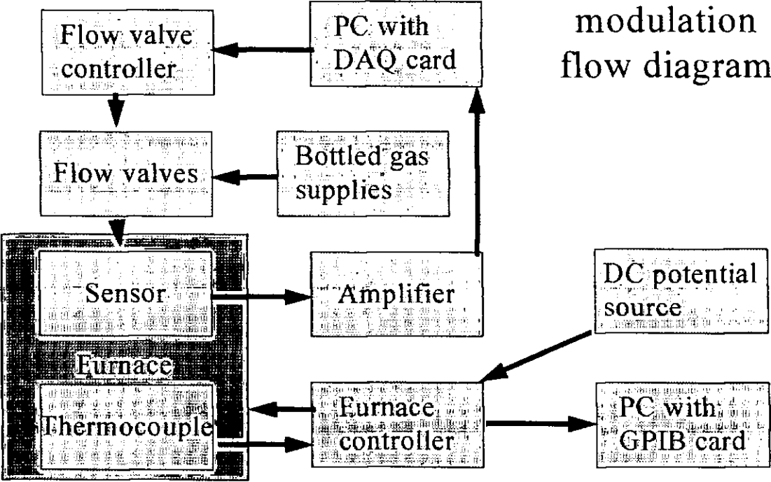
Figure C8 Concentration modulation configuration
