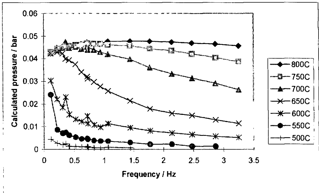
Figure 4.12 Pressure vs. modulation frequency, calculated from Equation 3.10
