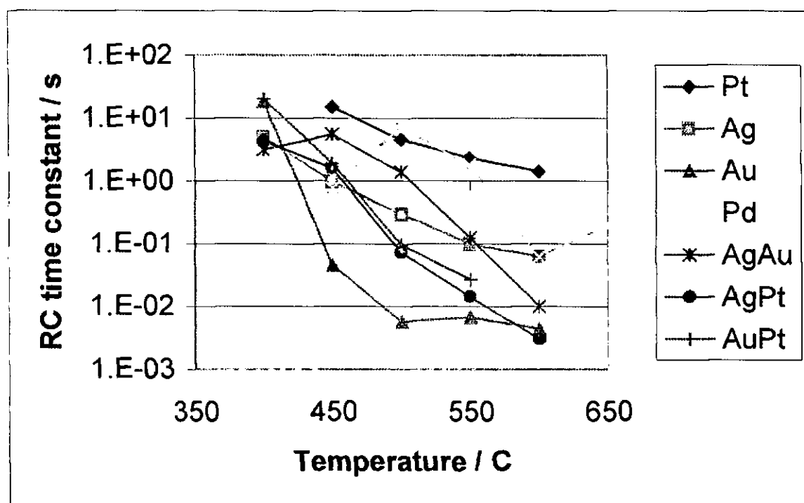
Figure 5.21 Electrode RC time constants calculated from individual R and C values obtained by frequency response analysis
