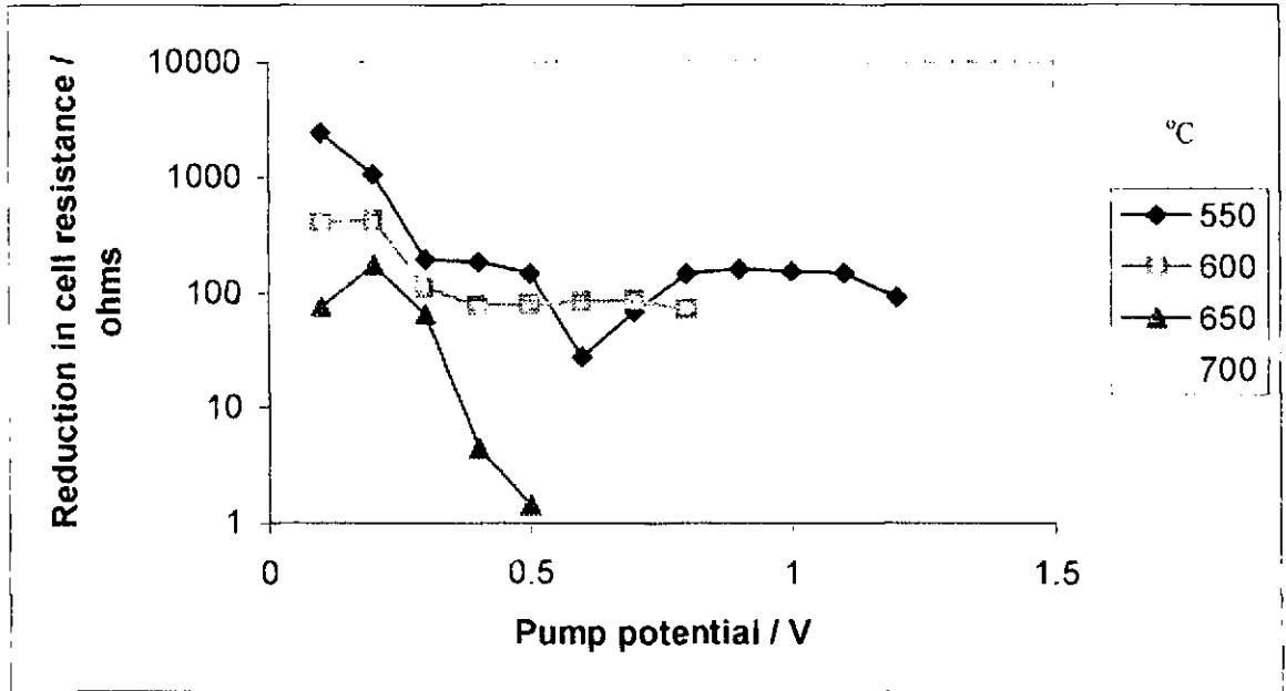
Figure F34 Post electro-deposit cell resistance improvements
