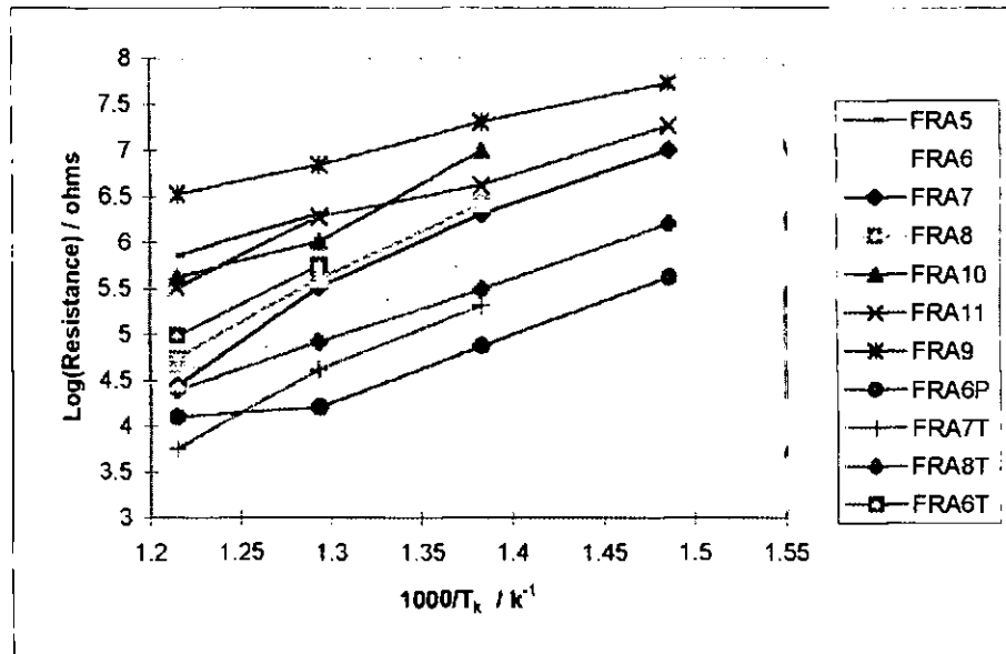
Figure 3.3 Arrhenius plot of electrode interface resistance for each electrode variation samples
