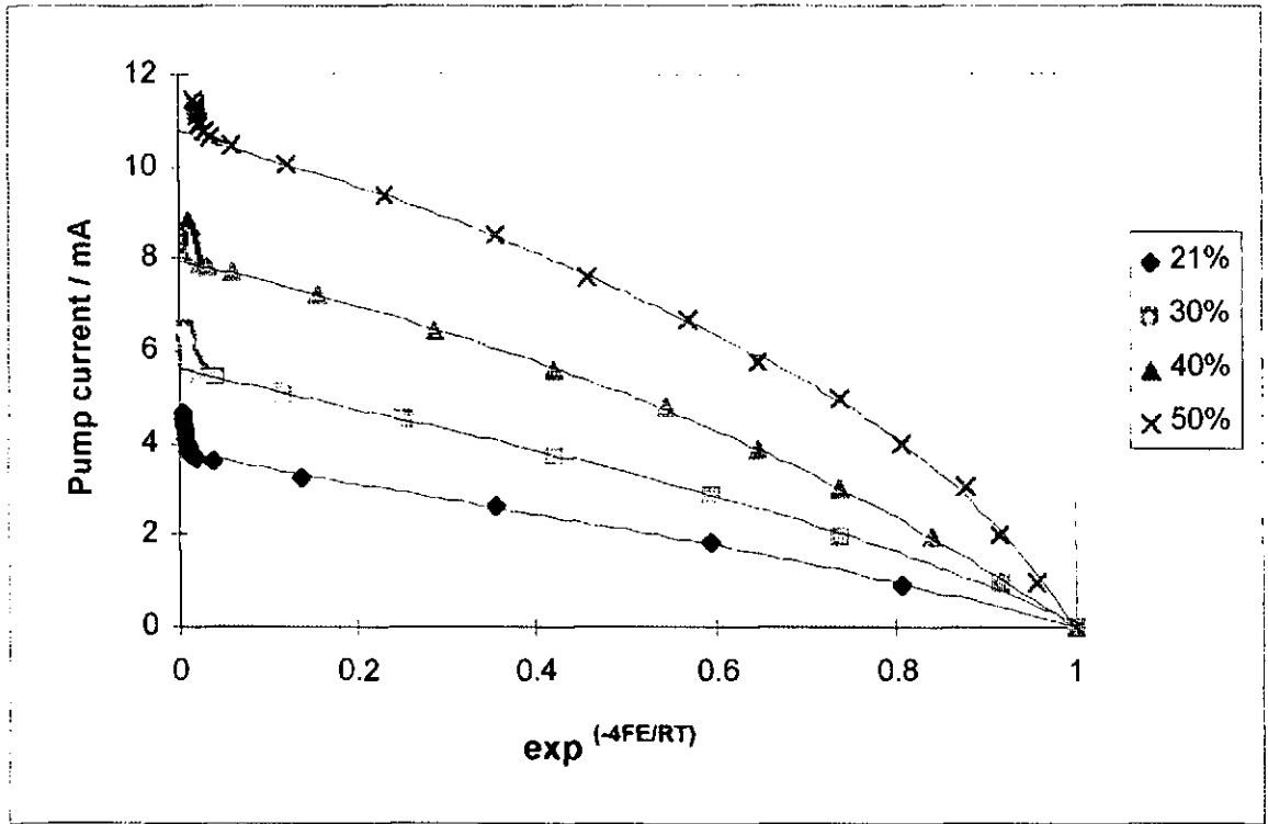
Figure F9 Exponential plot at high oxygen partial pressure
