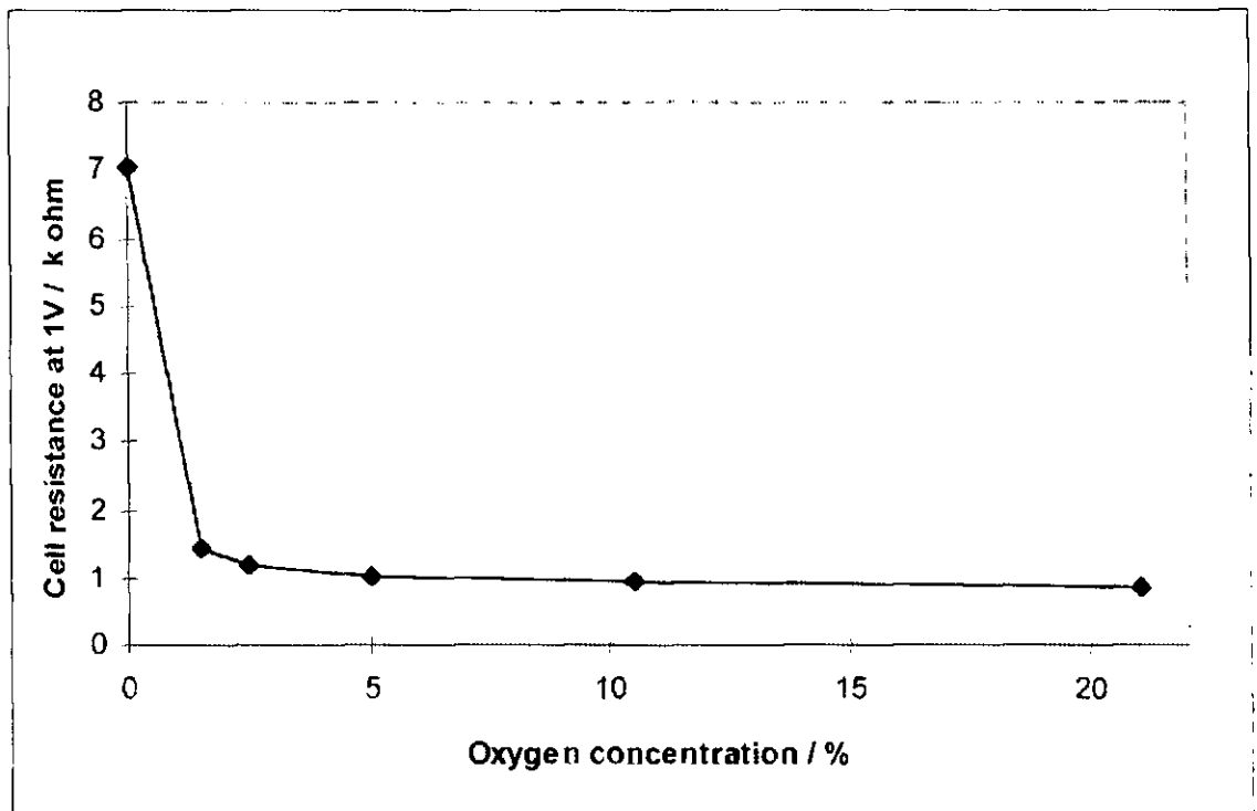
Figure F24 Cell resistance with oxygen concentration at 1 V pump potential
