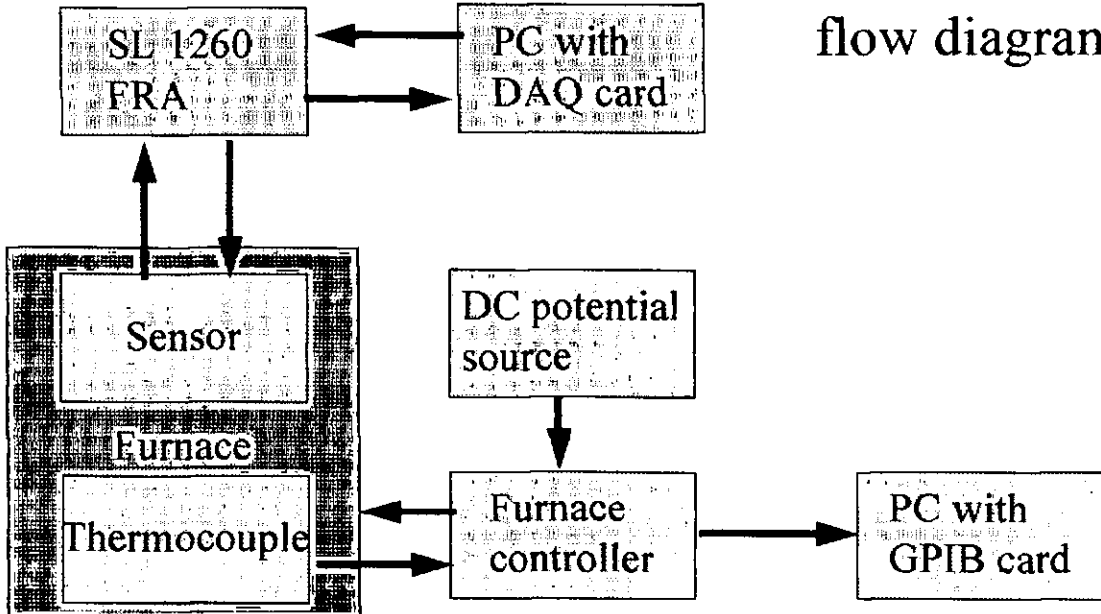
Figure C9 Frequency response configuration
