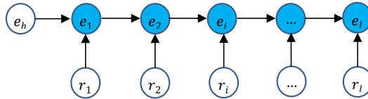
Figure 2: Generator modeling approach (latent states in blue, entities denoted e_i , relations, r_i )
