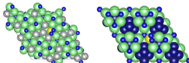
Figure 9. Graphic illustrating the adsorption of \text{N}_2 on a surface lattice N vacancy site for W-doped \text{Ni}_2\text{Mo}_3\text{N} ( \text{Ni}_{32}\text{Mo}_{59}\text{WN}_{28} ) (left) and W-doped \text{Co}_3\text{Mo}_3\text{N} ( \text{Co}_{52}\text{Mo}_{47}\text{WN}_{28} ) (right). Key: Ni, grey; Co, dark blue; Mo, green; W, yellow; N, pale blue.
