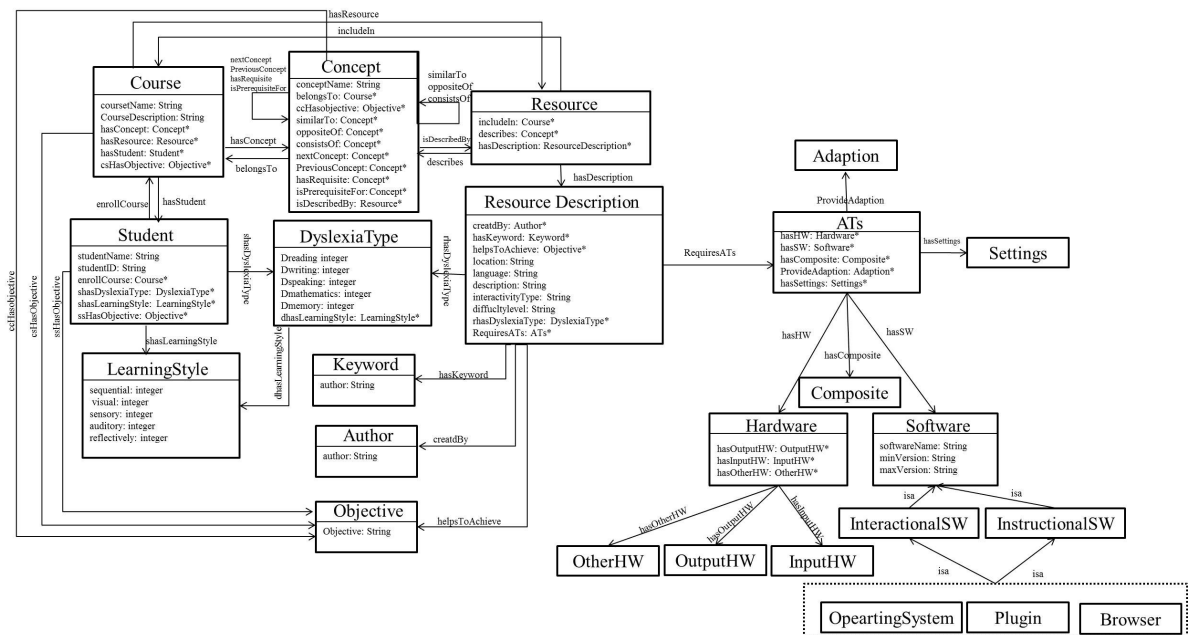
Fig. 1. General layout of the proposed ontology
