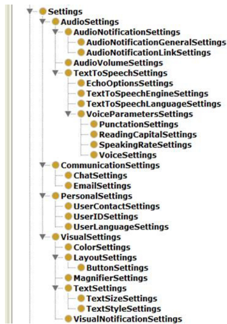
Fig. 3. Class Settings with its subclasses in Protégé
