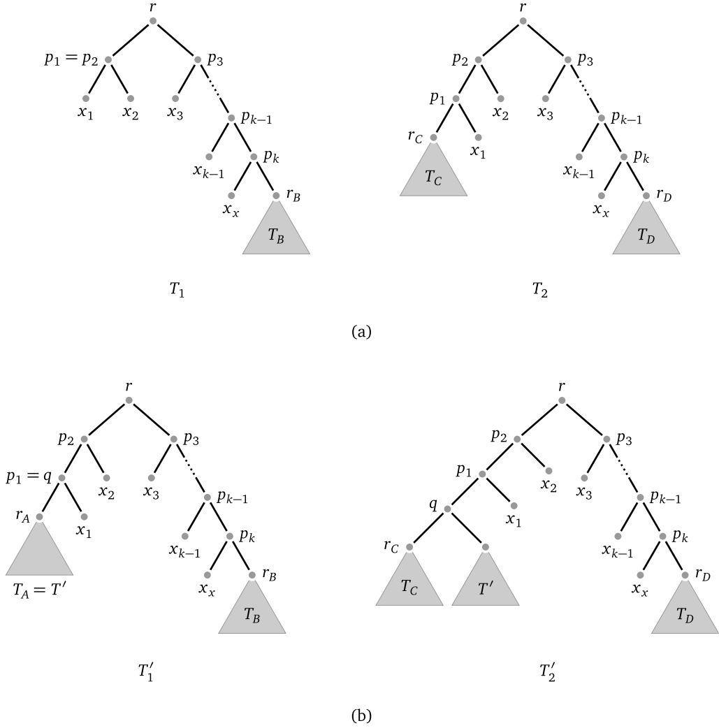
Fig. 4. (a) A common chain \langle x_1, \dots, x_k \rangle of T_1 and T_2 that is pendant in T_1 : T_A is empty. (b) The two trees T'_1 and T'_2 obtained by attaching a tree T_A = T' to T_1 and adding T' to T_C .
