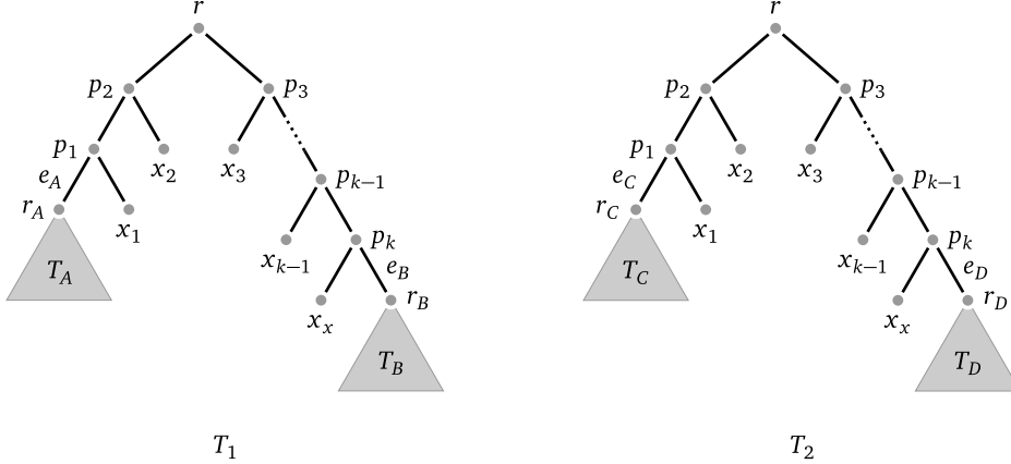
Fig. 3. The rooted versions of T_1 and T_2 considered for the discussion of chain reduction.
